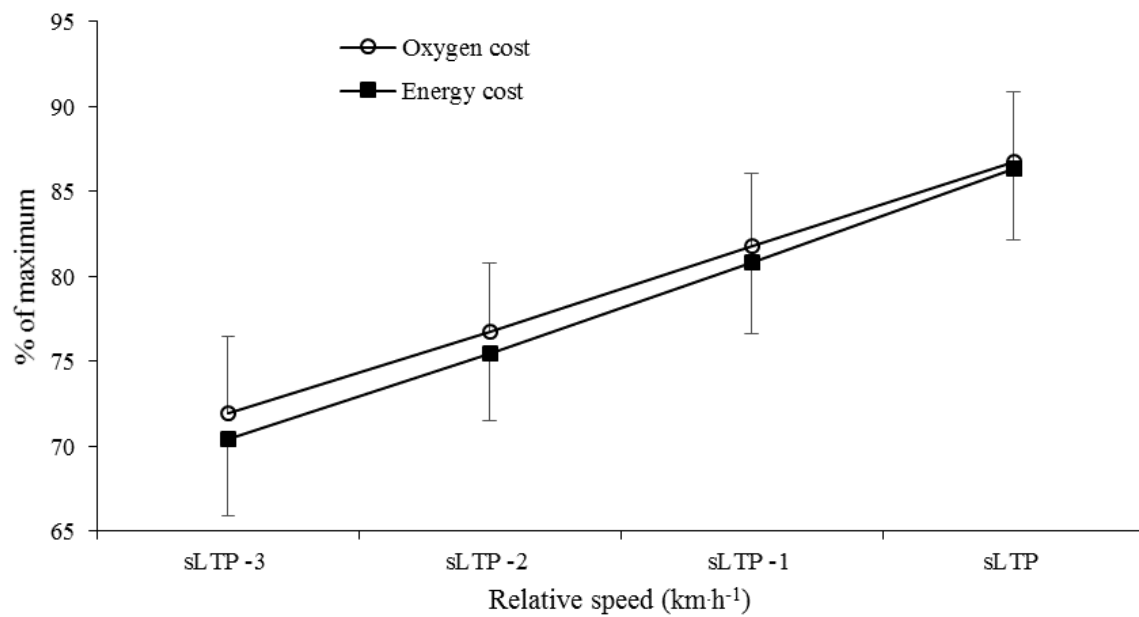
Fig. 3 Percentage utilization of maximum oxygen uptake and maximum aerobic energy expenditure across four sub-maximal relative speeds ( n = 56 ). sLTP = speed at lactate turn-point
