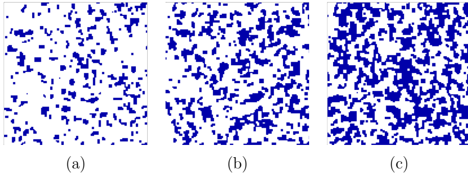
Figure 2. Melt ponds as metastable islands of like spins in our random field Ising model. Simulation results are shown for metastable states of the RFIM at H = 0 and J = 5 . The output spin configurations are shown on a 128 \times 128 portion of the 1024 \times 1024 lattice with (a) F_{out} = 0.15 ; (b) F_{out} = 0.30 ; (c) F_{out} = 0.45 . Pixels are colored blue for water ( s_i = +1 ) and white for ice ( s_i = -1 ).
