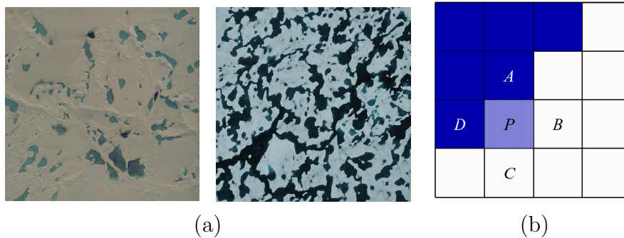
Figure 1. Melt pond configurations and the update step in Glauber dynamics. (a) Helicopter photos of melt ponds on sea ice in the western Beaufort Sea (D. Perovich). On the left, each side of this 15 July 1998 photo is 826 meters; on the right, each side of this 14 August 2005 photo is 193 meters. (b) Illustration of the tiebreaker update step in Glauber dynamics. Here each site i is assigned a pre-melt ice height h_i , and colored dark blue for water ( s_i = +1 ) and white for ice ( s_i = -1 ). Site P , to be updated, is adjacent to two water sites A and D , and two ice sites B and C . Since water tends to fill troughs, we require that s_P = +1 if h_P < 0 , and -1 otherwise.
