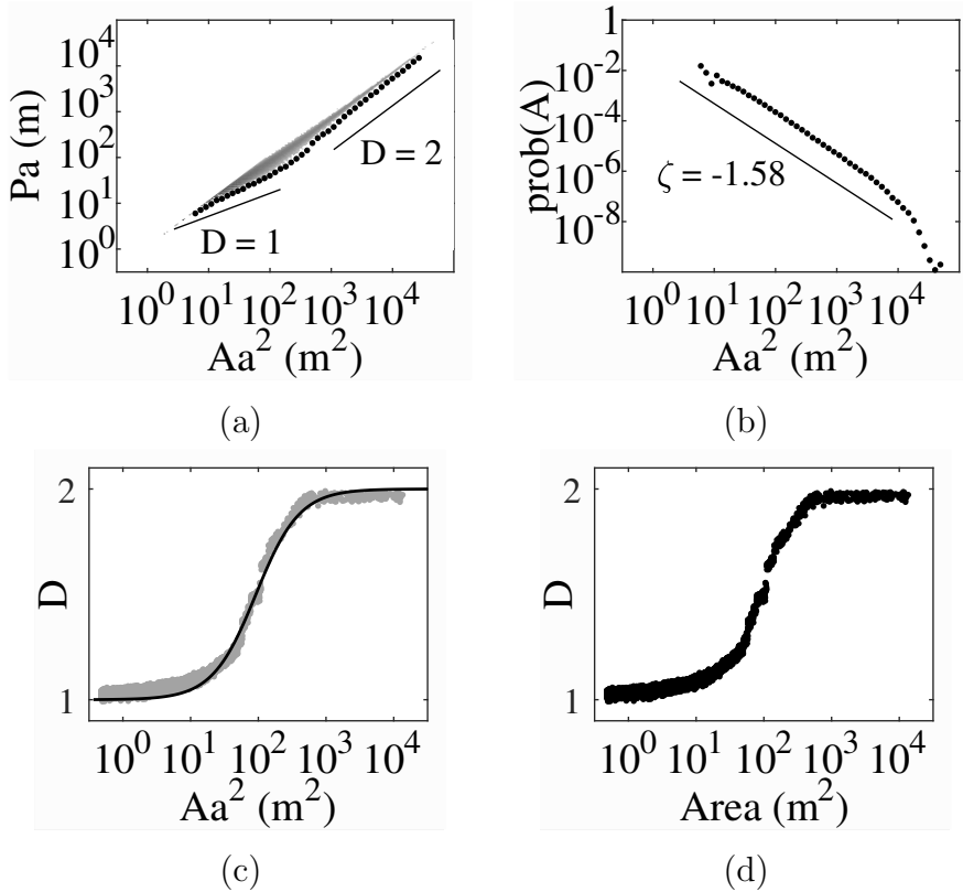
Figure 3. Geometrical characteristics of Ising model melt ponds. Simulation data in this figure are for the up-spin clusters in Fig. 2(c). (a) Log-log plot of the perimeter P versus the area A , rendered as a (rescaled) density plot. The lower edge of this cloud of points, highlighted by filled black circles, is determined by dividing \log(A) into bins of size 0.2 and computing the minimum of \log(P) for each bin. The reference lines have slopes 0.5 and 1, which correspond respectively to the fractal dimensions D = 1 and D = 2 . (b) Log-log plot of the pond size distribution function \text{prob}(A) , with bin size 0.2 and very small ponds with A < 5 \text{ m}^2 excluded. The reference line has slope -1.58 . (c) Plot of the fractal dimension D as a function of A (log scale) for our melt pond Ising model (thin solid curve) compared with the data curve (gray) for real melt ponds in (d) [10]. The solid curve is computed by fitting a suitable smooth function to the lower edge of the data points in panel (a) within the range 15 \text{ m}^2 < A < 400 \text{ m}^2 . (d) (Reproduced [10] with permission.) Fractal dimension as a function of area (log scale) based on image analysis of real melt ponds [10]. In panels (a)-(c), A and P are shown in physical units with the lattice constant a = 1 \text{ m} , and the number of sites is increased to 8192 \times 8192 to improve the statistics.
