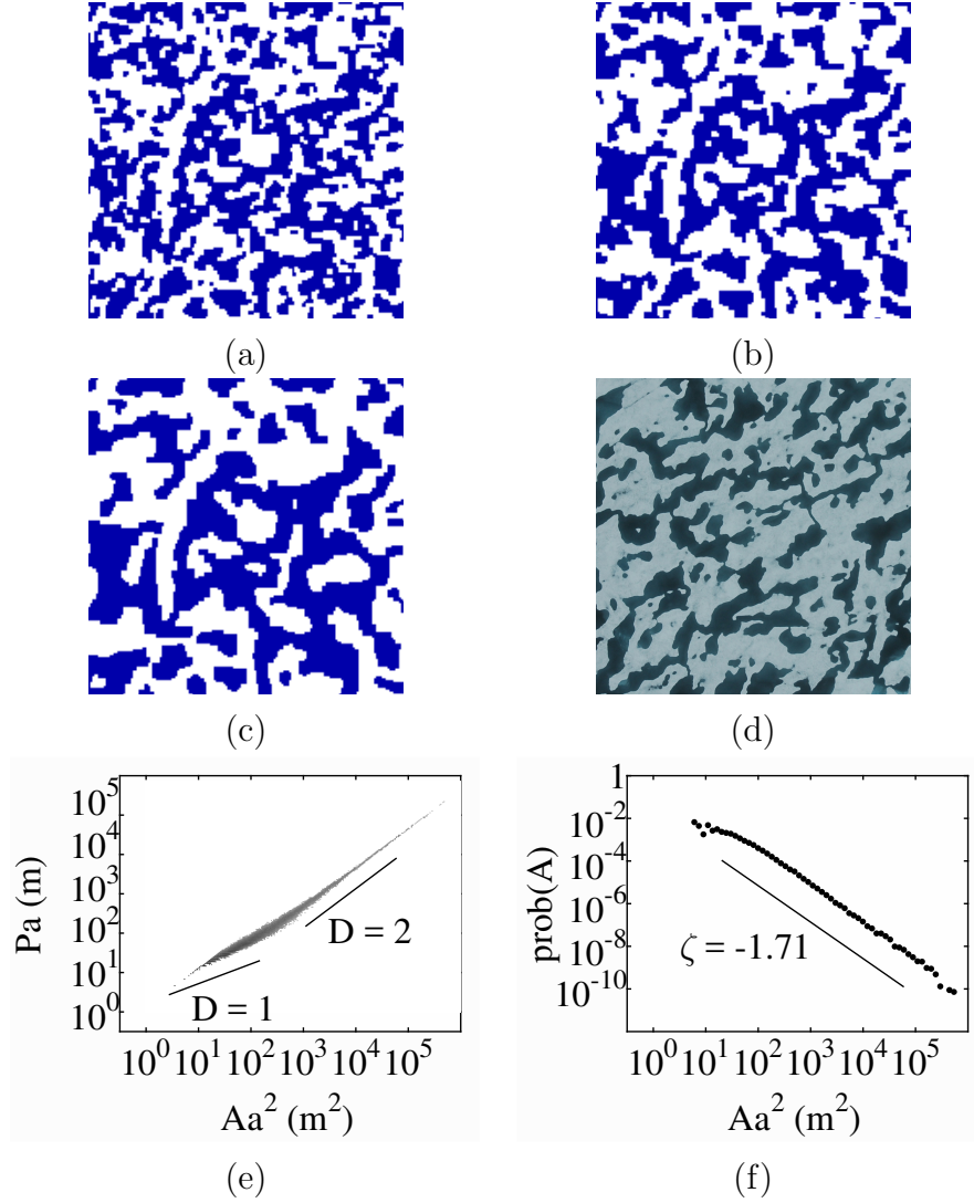
Figure 4. Time evolution of metastable states with an evolving ice topography. Simulation results are shown for metastable states of the RFIM at H = 0 and J = 10 . The h_i^n at n = 0, 1, 2, \dots are assumed to be independent Gaussian variables with zero mean and unit variance. The input configuration s_i^0 has pond fraction F_{in} = 0.495 . The output configurations s_i^n are shown on a 165 \times 165 lattice at (a) n = 2 ; (b) n = 4 ; (c) n = 8 . Pixels are colored blue for water ( s_i = +1 ) and white for ice ( s_i = -1 ). (d) Aerial image of Arctic melt ponds. Each side of this photo is 165 meters. Panels (e,f) show the geometric characteristics of the up-spin clusters in panel (b). (e) Log-log plot of the perimeter P versus the area A , rendered as a (rescaled) density plot. The reference lines are at the same location as those in Fig. 3(a) to facilitate comparison. (f) Log-log plot of the pond size distribution function \text{prob}(A) , with bin size 0.2 and very small ponds with A < 5 \text{ m}^2 excluded. The reference line has slope -1.71 .
