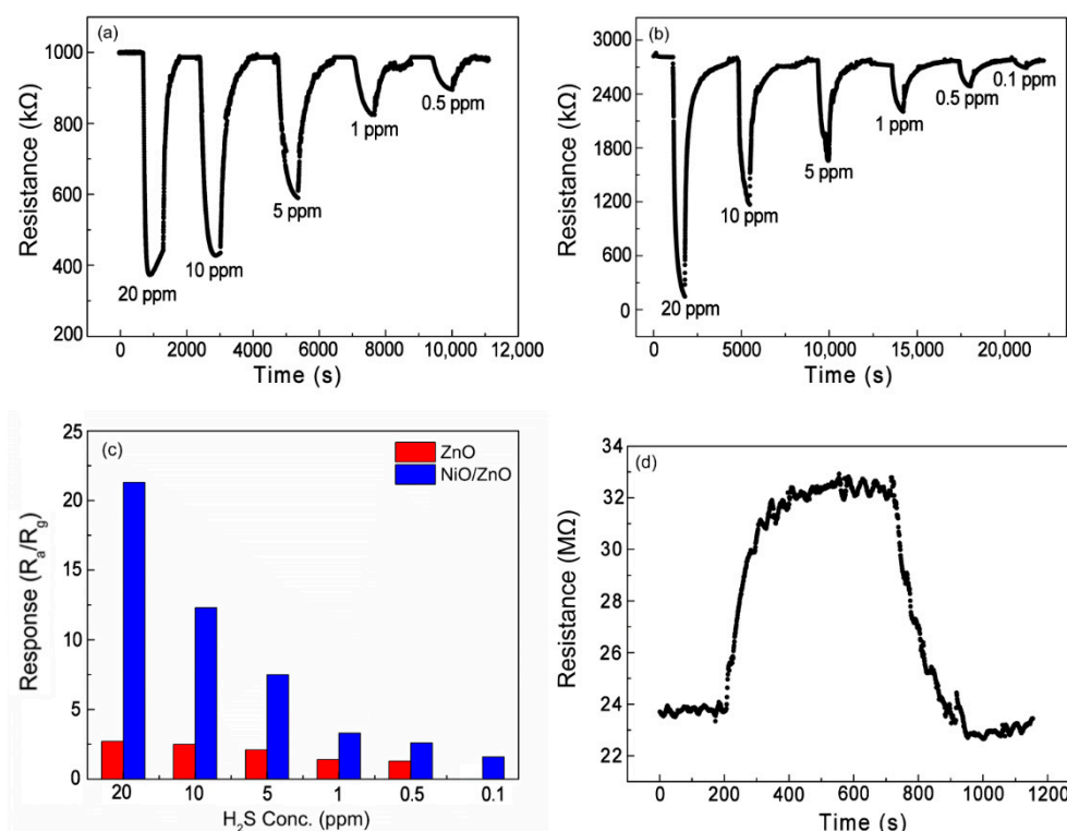
Figure 7. Dynamic response curves upon exposure to H_2S with different concentrations at 160\text{ }^\circ\text{C} exhibited by sensors based on: (a) pure ZnO NRs and (b) NiO/ZnO, and (c) responses histogram of sensors and (d) pure NiO NSs.
