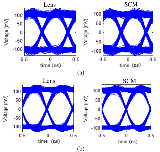
Fig. 5 The eye diagrams of the received signals obtained when Lens or SCM was used at the visibilities of: (a) 0.062 km, and (b) 0.080 km.
