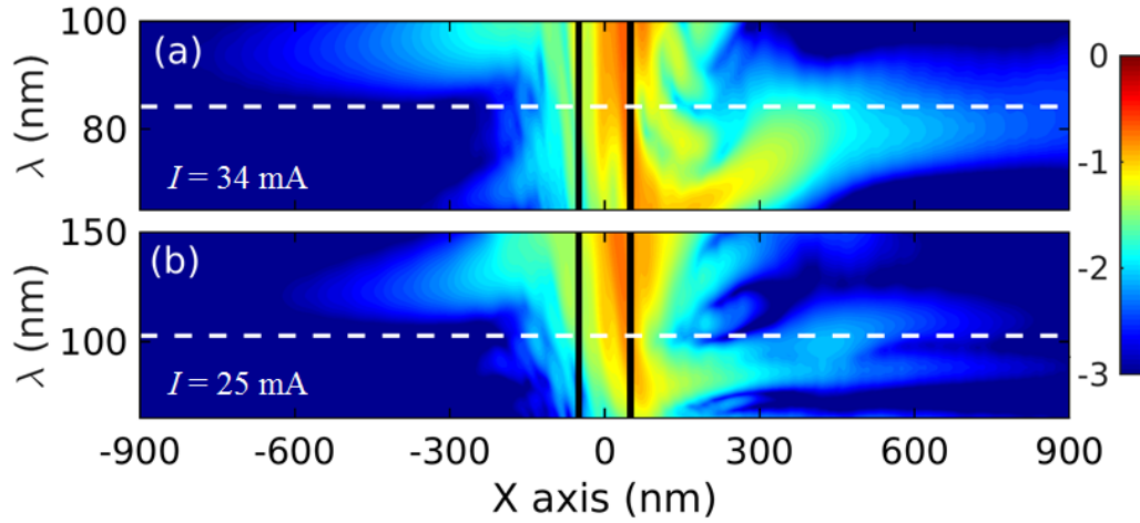
Figure 6 (color online) Smoothed pseudo-Wigner-Ville transform of simulated SWs along X for (a) I = 34 mA and (b) I = 25 mA and an external field of H = 800 mT. The vertical black lines indicate the boundaries of the NC while the white dashed lines indicate wavelength obtained from the spin wave dispersion relation at each frequency, namely, (a) 19.2 GHz and (b) 17.1 GHz. The color contrast indicates the normalized magnitude in logarithmic scale of the SW associated with each wavelength (y axis) as a function of X.
