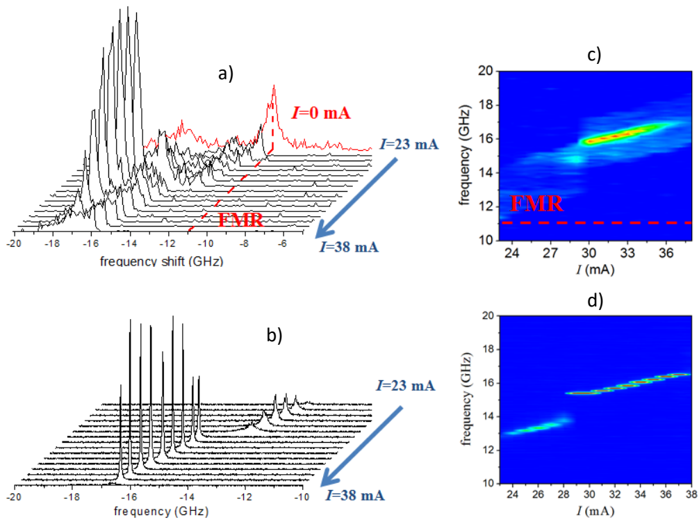
Figure 4 (color online). (a) \mu -BLS and (b) SA spectra measured as a function of the intensity of the injected DC ( I ) for a fixed value of the external field H = 680 mT. (c) and (d) color plots of the sequence of spectra (a) and (b).
