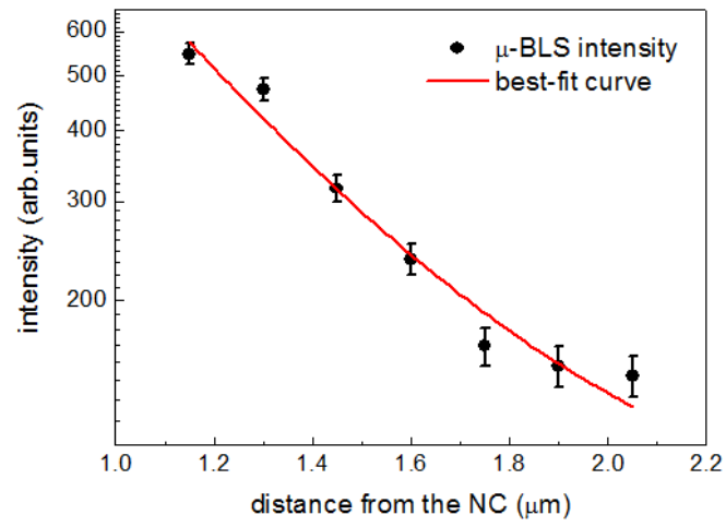
Figure 2 (color online). (circles) Spin-wave intensity measured by \mu -BLS as a function of the distance ( X-X_0 ) from the NC position. (line) Best-fit curve obtained using expression (1).
