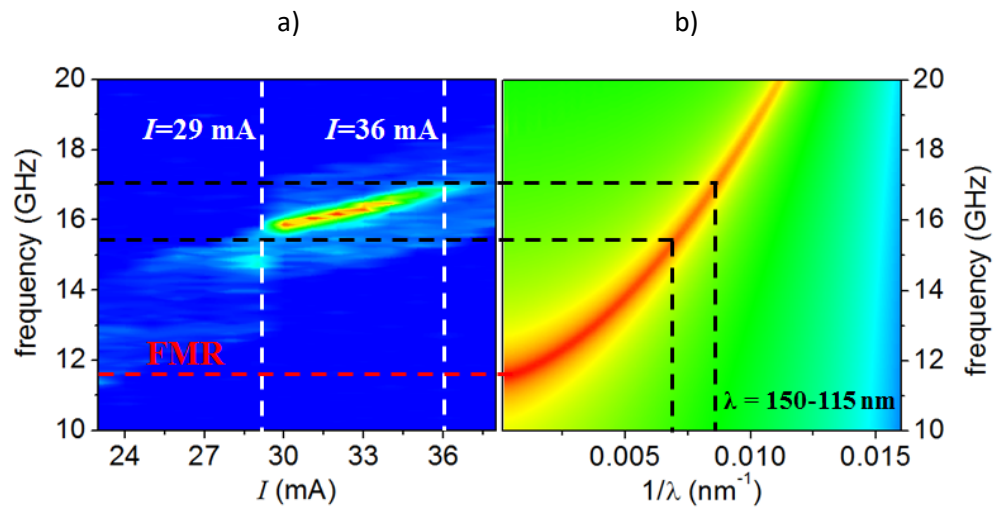
Figure 5 (color online). (a) \mu -BLS spectra measured as a function of the intensity of the injected DC ( I ) for a fixed value of the external field H = 680 mT. (b) Simulated SWs dispersion curve of the NiFe free layer.
