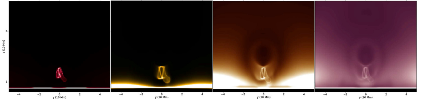
Figure 4. Synthetic SDO/AIA views at t = 150 minutes. The wavelength and peak temperature are from left to right: 304 \text{ \AA} (0.08 MK), 171 \text{ \AA} (0.8 MK), 193 \text{ \AA} (1.5 MK), and 211 \text{ \AA} (1.8 MK). In the latter two wavelengths, we see prominence horns and a central dark cavity.
