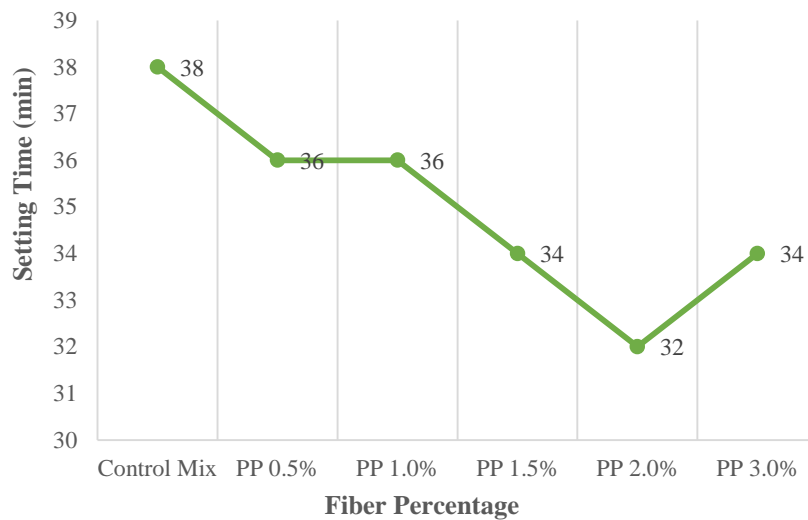
Figure 3: Initial setting time variation
