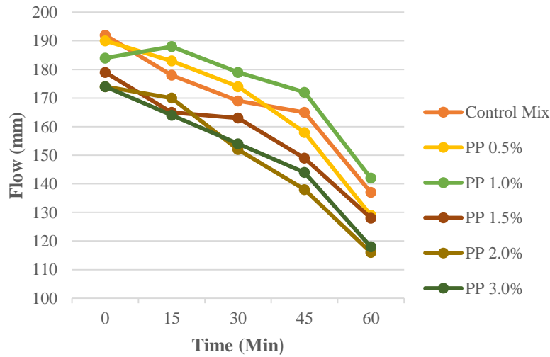
Figure 2: Loss of workability with time of the mix with different fibre percentage
