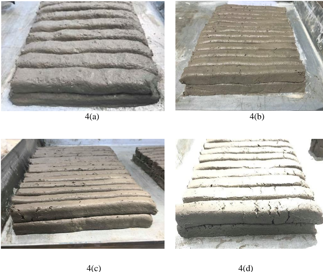
Figure 4: (a) Extruded specimen of PP 0.5%, (b) Extruded specimen of PP 1.0%, (c) Extruded specimen of PP 1.5%. (d) Extruded specimen of PP 2.0%
