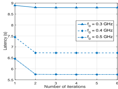
Fig. 2. Latency versus number of iterations with different local computing capacity f_0 .
