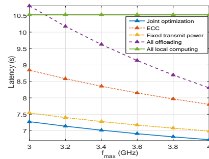
Fig. 3. Latency versus the maximum MBS computing capacity f_{max} .
