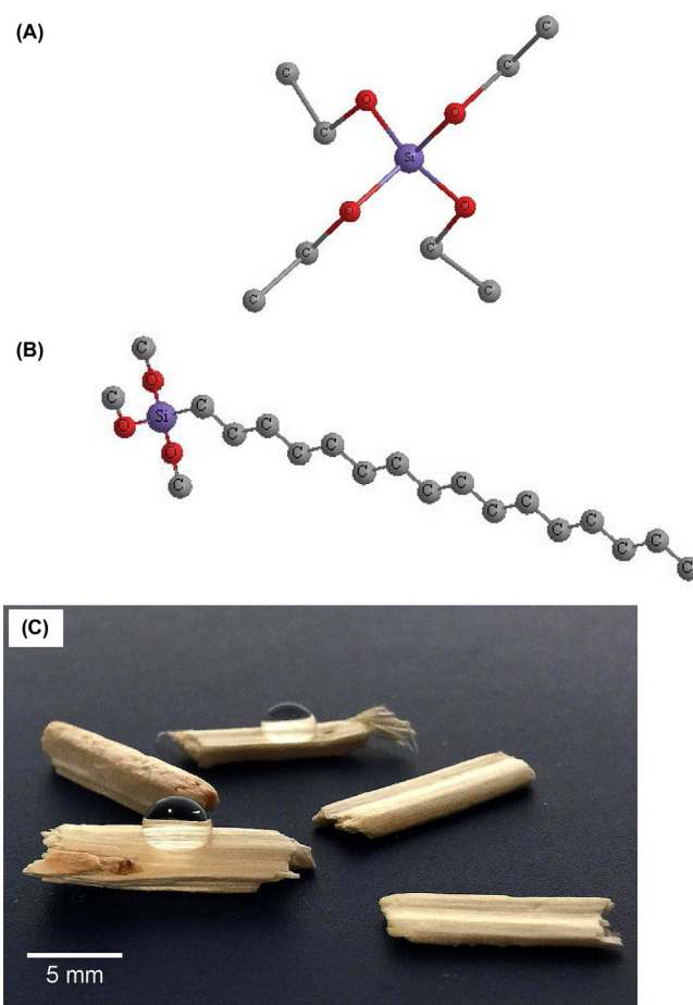
Fig. 1. 3D structure of a (A) TEOS molecule, (B) HDTMS molecule; and (C) water on coated hemp shiv samples.
