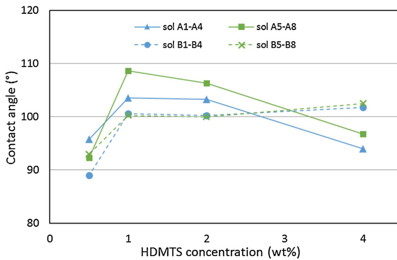
Fig. 3. Effect of ethanol dilution and varying HDTMS concentration in the sol-gel coating on hydrophobicity of hemp shiv surface.
