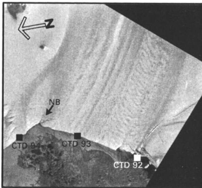
Figure 2. A March 15, 1994, ERS-1 SAR (synthetic aperture radar) satellite image of the western end of PIG. The northern boundary of the calving front is shown by the NB arrow, and the southern boundary is near CTD 92, located at 75^{\circ}03.6\text{S} , 101^{\circ}50.8\text{W} . The PIG floats above a 70-90 km-long cavity with a draft ranging from <340 m at the ice front to >1200 m near the grounding line [Crabtree and Doake 1982; Jenkins et al. subm. ].
