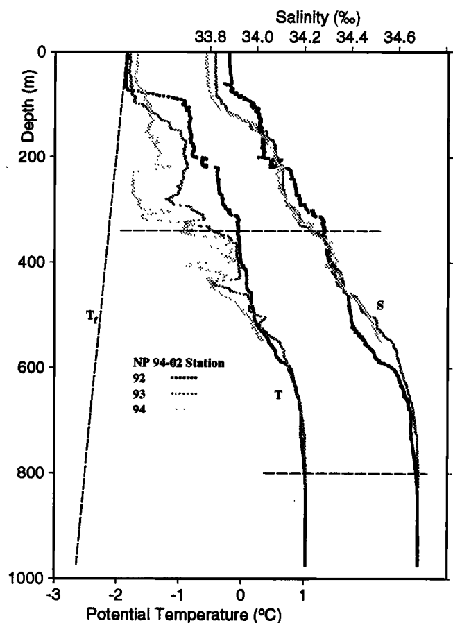
Figure 3. Potential temperature and salinity vs. depth on stations 92-94, taken near the PIG (Figure 2) on March 14, 1994. Horizontal dashed lines show the 340 m draft of PIG (Figure 4) and the 800 m division between deep inflow and shallower outflow. Water below 800 m is >3^{\circ}\text{C} warmer than the in-situ freezing temperature ( T_f ).
