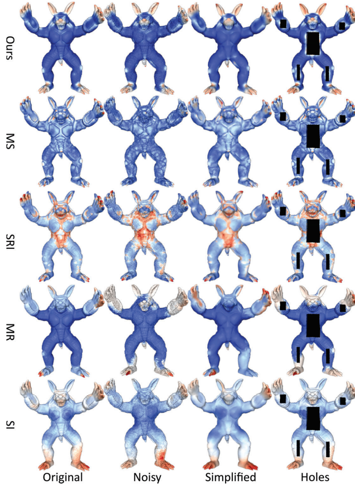
Figure 8: Comparison of the robustness of our method with that of others. The columns from left to right correspond to the original Armadillo mesh, the noisy version (20% noises in vertex normal directions), the simplified version (with 5k vertices), and the broken version with holes. The competing methods are MS [6], SRI [18], MR [19], and SI [9].
