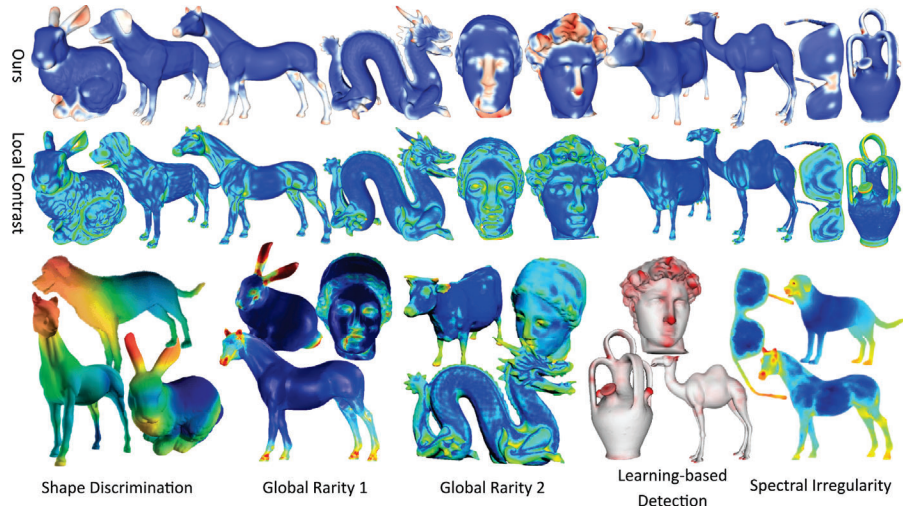
Figure 5: Comparison of our saliency maps with that generated by other methods. The competing methods include Local Contrast [6], Shape Discrimination [7], Global Rarity 1 [18], Global Rarity 2 [19], Learning-based Detection [20], and Spectral Irregularity [9]. Following [18, 19, 9], we take the rendered saliency maps from the original papers of [18, 19, 9, 7, 20] because we do not have access to their source codes. For the method of [6], we generate the saliency maps using our own implementation and visualize them to match the original color themes.
