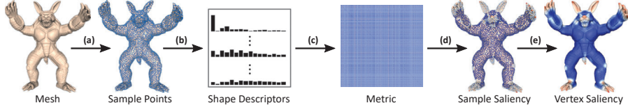
Figure 1: Overview of our sparse metric-based mesh saliency detection method. The steps from (a)-(e) are mesh sampling, shape descriptor construction, metric computation, saliency optimization, and vertex saliency interpolation respectively. We use red and blue colours to indicate high and low saliency values respectively.
