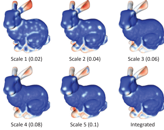
Figure 3: Multi-scale saliency integration. The saliency map of each scale is computed from the corresponding metric and the integrated map is computed from the sum of the metrics of all scales.
