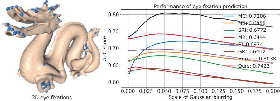
Figure 6: Performance of eye fixation prediction. Left: The Dragon and our captured ground-truth 3D eye fixations on the surface. Right: The Human method uses the captured eye fixations of half subjects to predict that of the other halves, thereby measuring the self-consistency of our eye fixation dataset. The competing methods are MC [51], MS [6], SRI [18], MR [19], SI [9], and GR [8]. The peak AUC scores of these methods are displayed in the plot legend.
