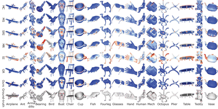
Figure 7: Comparison of the saliency maps generated on the dataset of [20]. The first six rows correspond to the competing methods of MS [6], SRI [18], MR [19], SI [9], and GR [8]. The seventh row is our proposed method and the eighth shows the ground-truth salient points (in blue) and saliency distributions (in red). The columns correspond to the 19 categories (excluding Helix as in the original paper) of the dataset of [20]. Please zoom in to compare the details of the saliency maps.
