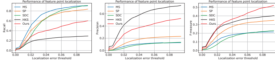
Figure 9: Performance of feature point localization on the dataset of [22] . Four competing methods that are highly cited in the field are included: MS [6], SP [24], SDC [23], and HKS [25]. We use the popular Recall, Precision, and F-measure for performance evaluation [22].
