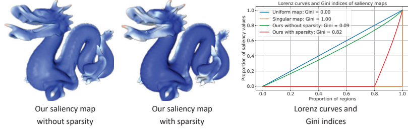
Figure 2: Saliency detection with and without sparsity. Left: our computed saliency map without sparsity. Middel: our computed saliency map with sparsity. Right: Lorenz curves and Gini indices of saliency maps. Our map without sparsity is both visually and quantitatively similar to the uniform one, while our map with sparsity is quantitatively sparser and visually more concentrated on distinct regions .
