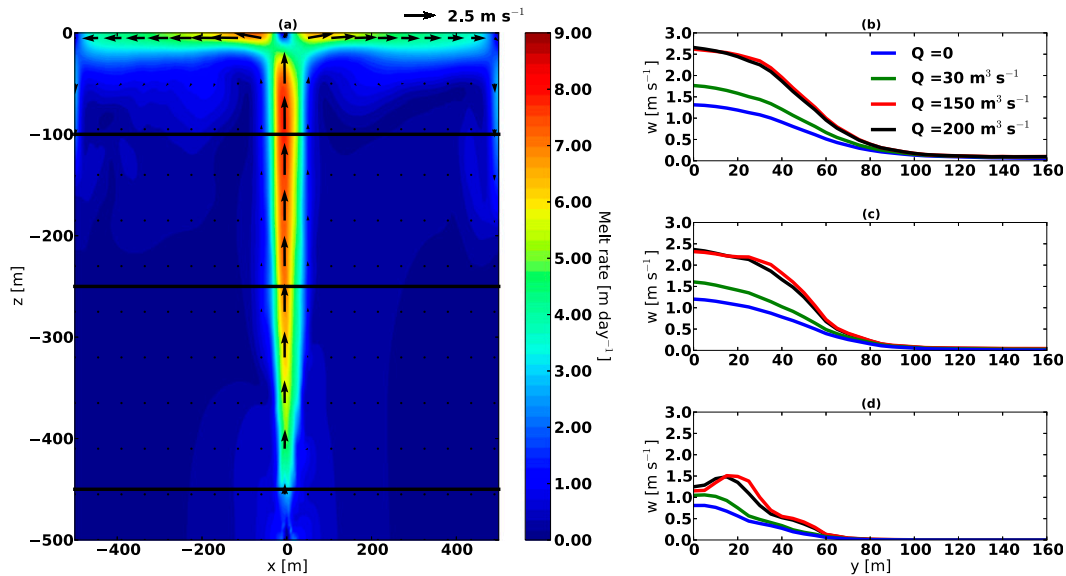
FIG. 5. (a) Distribution of temporally averaged melt rate and velocity vector, u and w for d \times h = 10 \times 10 m at Q = 150 \text{ m}^3 \text{ s}^{-1} . Velocity vectors are projected onto a structured grid that has a horizontal and vertical resolution of 55 and 45 m, respectively. Profiles of vertical velocity along the center of the channel ( x = 0 ) for different Q at selected depth: (b) z = -100 m, (c) z = -250 m, and (d) z = -450 m. Solid lines in (a) indicate the depth at which profiles (b), (c), and (d) are taken.
