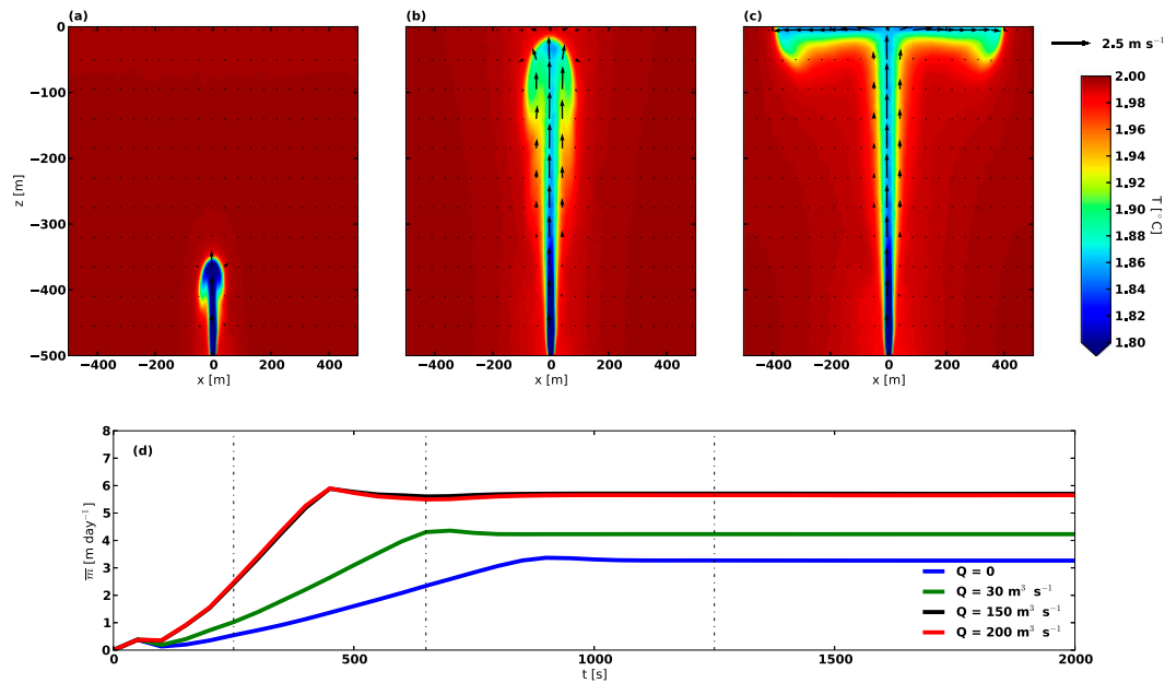
FIG. 4. Snapshots of instantaneous temperature field and velocity vectors, u and w , on the vertical ice face ( y = 0 ) for Q = 30 \text{ m}^3 \text{ s}^{-1} at (a) t = 300 s, (b) t = 700 s, and (c) t = 1300 s. Velocity vectors are projected onto a structured grid that has a horizontal and vertical resolution of 45 m. (d) Evolution of \bar{m} (m day -1 ) for different values of Q from d \times h = 10 \text{ m} \times 10 \text{ m} . Vertical dashed lines in (d) indicate the time in which the snapshots are taken.
