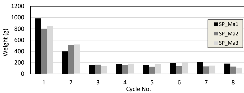
Figure 20. Weight of absorbed water (masonry specimens).
