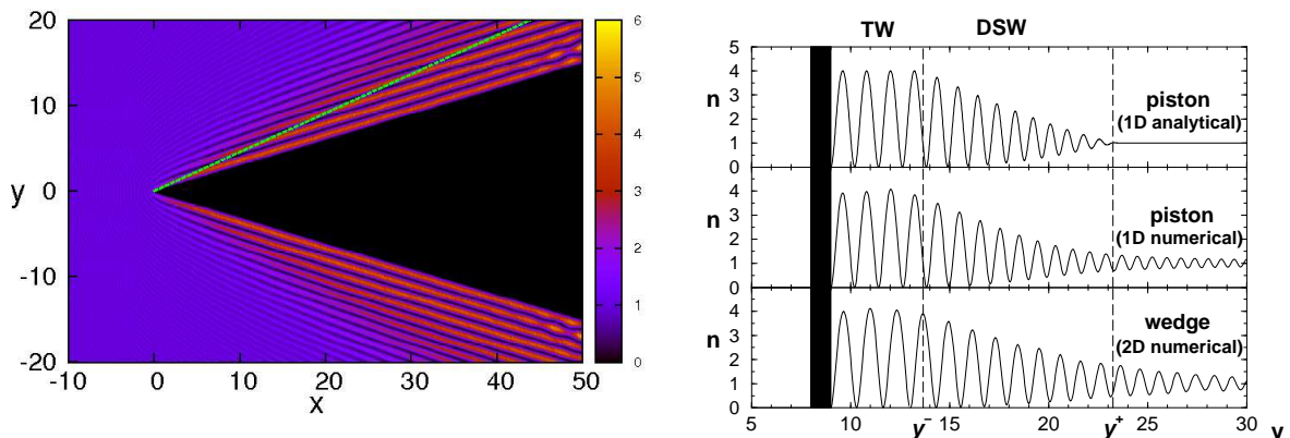
FIG. 13: Left (color online): 2D density plot for the supersonic M = 10 NLS flow past a wedge with the opening angle above the x -axis \alpha = 0.3 . The dashed line marks the end of the transition wave predicted by the theory. Right: density profile n(y) at x = 30 ; top: analytical modulated solution; middle: numerical solution of the associated 1D piston problem; bottom: 1D cut of the full 2D solution at t = 15 . Points y^- and y^+ mark the boundaries of the DSW specified by the modulation solution. The body surface (piston) is located at about y = 9 .
