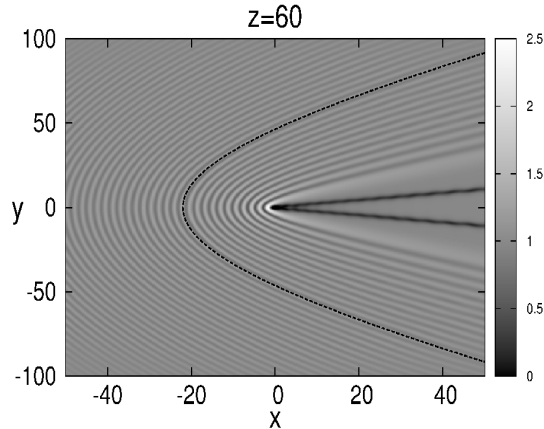
FIG. 5: Numerically calculated wave pattern corresponding to diffraction of a light beam on the obstacle embedded into a photorefractive medium. The plot corresponds to \gamma = 0.2 , U = 2 , and the radius of the reflecting wire to r = 1 . Dashed line corresponds to linear analytical theory, Eq. (37), for the line of constant phase; it is shifted to the left to two units of length from the center of the obstacle due to its finite size in numerical simulations and better fitting to numerics.
