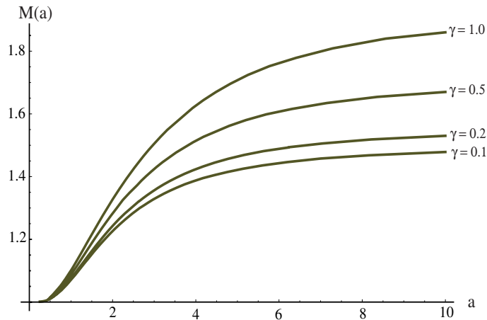
FIG. 10: Boundary between regions of absolute and convective instabilities for several values of the saturation parameter \gamma .
