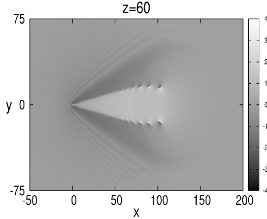
FIG. 3: Distribution of the phase in the diffraction pattern at the output plane of the photorefractive medium. The pattern corresponds to \gamma = 0.2 , U = 2 , and z = 60 .
