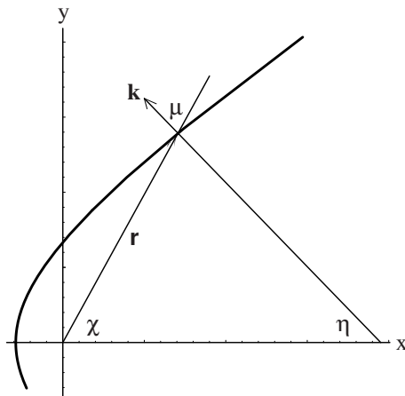
FIG. 4: Coordinates defining a radius vector \mathbf{r} and a wave vector \mathbf{k} , normal to the wave front shown schematically by a curved line.
