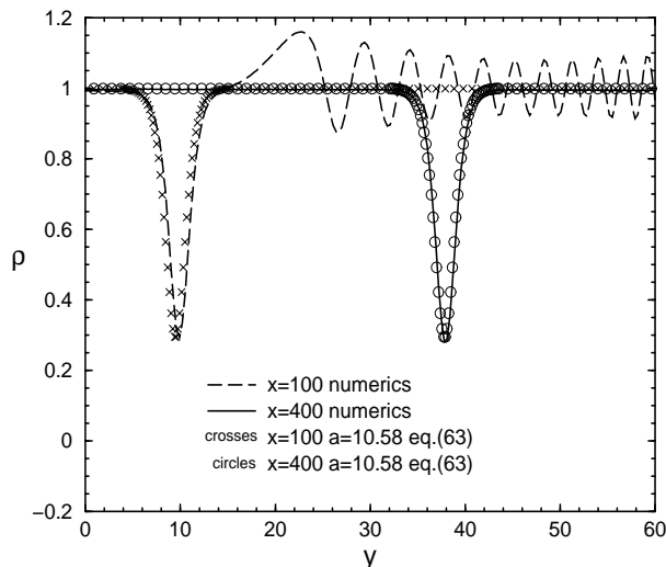
FIG. 8: Profiles of the intensity distributions for x = 100 (dashed line), x = 400 (solid line) and y > 0 obtained from numerical solution of the equation (5) with the nonlinear term given by (6). These profiles are compared with the soliton profiles obtained by solutions of Eq. (63) with slope a = 10.58 shown as functions of y at the same values of x ( x = 100 corresponds to “crosses” and x = 400 to “circles”).
