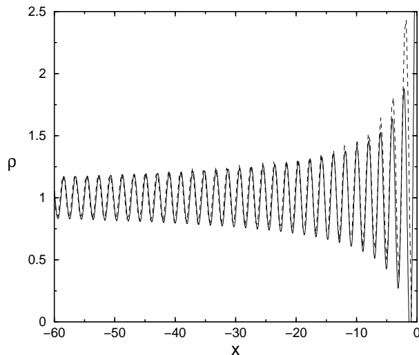
FIG. 6: Profile of intensity in front of the the obstacle for x < 0 , y = 0 and choice of the parameters \gamma = 0.2 , U = 2 , V_0 = 2.4 . Solid line corresponds to Eq. (42) and dashed line to numerical solution of Eqs. (5,6).
