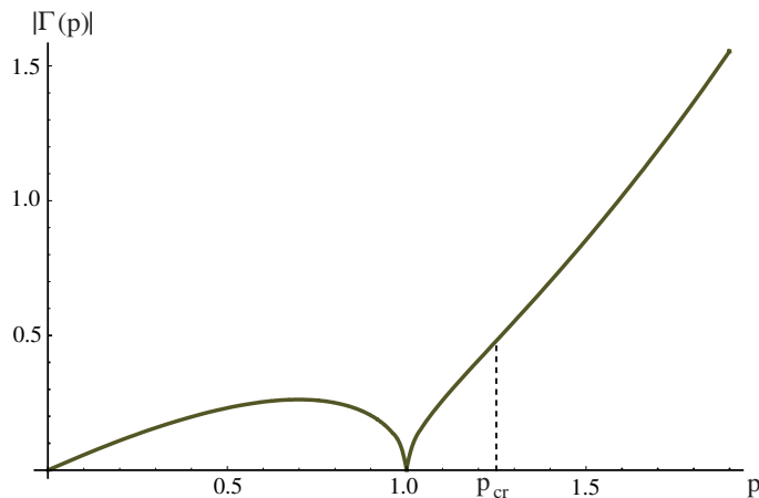
FIG. 9: Absolute value of the growth rate \Gamma as a function of the wave number p of a harmonic transverse perturbation for \gamma = 1 and \rho_m = 0.2 .
