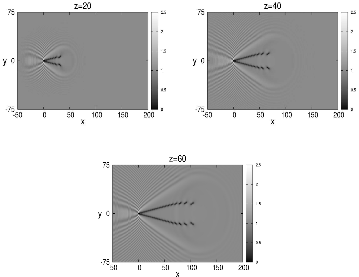
FIG. 2: Evolution of the diffraction pattern at the output plane as a function of the length z of the photorefractive medium. The patterns are obtained by numerical solution of Eq. (4) with V(\mathbf{r}) corresponding to an ideally reflecting wire with unit radius for \gamma = 0.2 , U = 2 , and (a) z = 20 , (b) z = 40 , (c) z = 60 .
