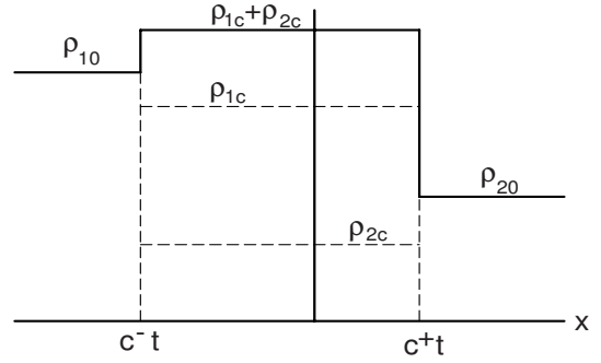
FIG. 1: Dependence of solitons densities on space coordinate x at some moment t ; \rho_{10} and \rho_{20} are the densities of solitons in the beams propagating to the left and to the right, correspondingly; \rho_{1c} and \rho_{2c} are the densities of the same beams in the overlap region.
