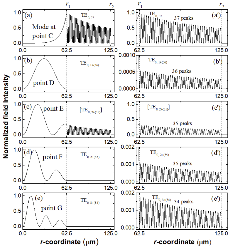
Fig. 4. The left panel (a)-(e) shows the normalized intensity distributions along the r -coordinate for the modes shown at points C-G in Fig. 3. The right panel (a')-(e') shows the zoomed-in part of (a)-(e), delineated by the vertical dashed lines.
