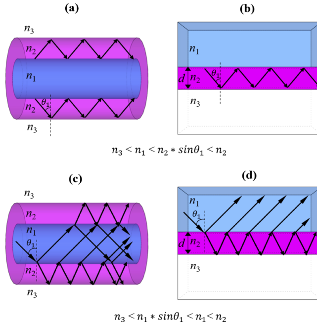
Fig. 2. (a) and (b) show the ray trajectory of a mode with n_1 < n_{\text{eff}} = n_2 \sin\theta_1 < n_2 in a DCF and an equivalent asymmetric planar waveguide, respectively. (c) and (d) show the ray trajectory of a mode with n_3 < n_{\text{eff}} = n_1 \sin\theta_1 < n_1 in the DCF and the equivalent asymmetric planar waveguide, respectively.
