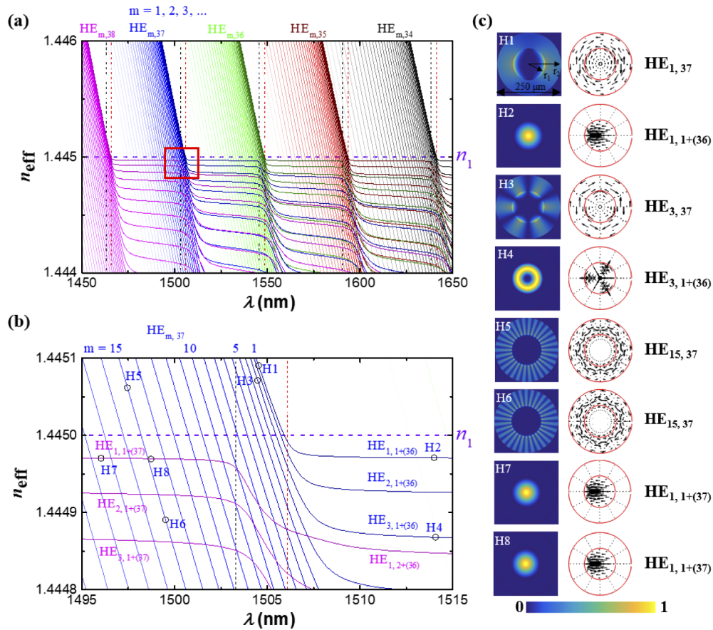
Fig. 7. Dispersion curves ( n_{\text{eff}} vs. \lambda ) of HE modes with n_{\text{eff}} corresponding to (a) n_1 - 0.001 < n_{\text{eff}} < n_1 + 0.001 , n_1 = 1.445 . (b) partially enlarged image of (a), indicated by the red frame. (c) shows the modal intensity and electric field vector distributions of HE modes whose positions ( n_{\text{eff}} , \lambda ) are indicated by the circles in (b). The black and red vertical dashed lines in (a) and (b) indicate the resonant bands.
