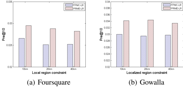
Figure 4: Different localized region constraint on two datasets.
