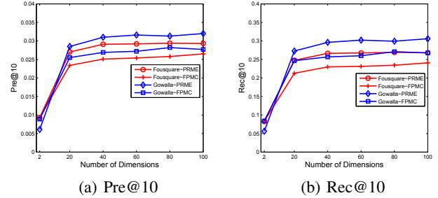
Figure 7: Effect of the number of dimension for PRME.
