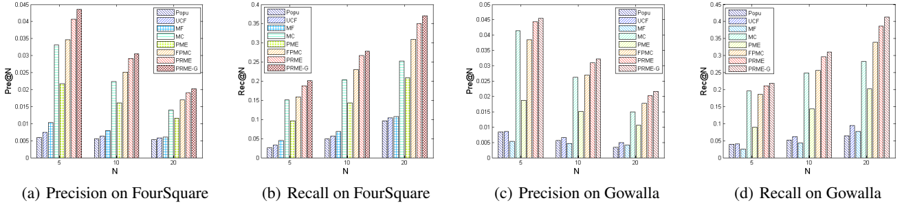
Figure 3: The result of methods on Foursquare and Gowalla.
