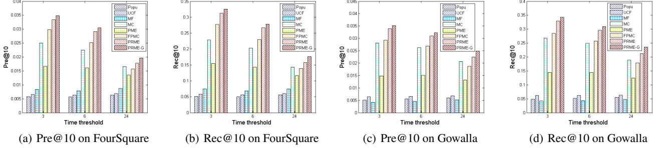
Figure 5: The effect of time threshold \tau on Foursquare and Gowalla.
