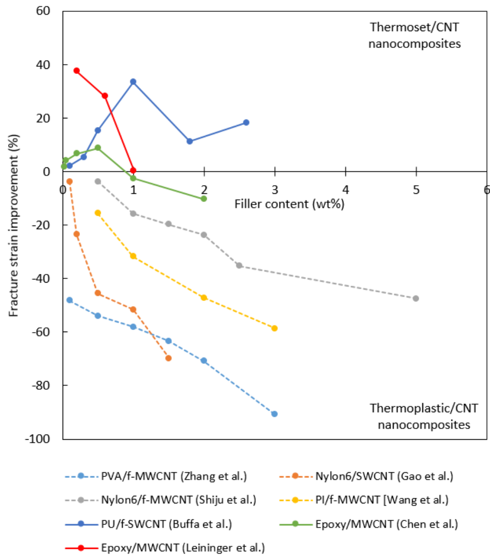
Figure 13: Fracture strain improvement of CNT based polymer nanocomposites as a function of filler content (Adapted from [94, 96, 109, 110, 239-241])
