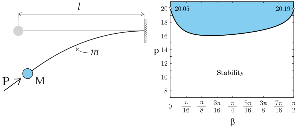
Fig. A The Pflüger column and its stability diagram. The ratio of the end mass to the mass of the column, \mu = M/(ml) , is parameterized by \mu = \tan\beta . The Beck column corresponds to the vanishing end mass ( M = 0 , so \beta = 0 ) and the massless Pflüger column (or Dzhanelidze's column (6)) to the vanishing mass of the rod ( m = 0 , so \beta = \pi/2 ). The vertical axis of the stability diagram shows the dimensionless load p = \frac{Pl^2}{EI} , where E is Young's modulus, I is the moment of inertia of a cross-section of the column and l is the length of the column.
