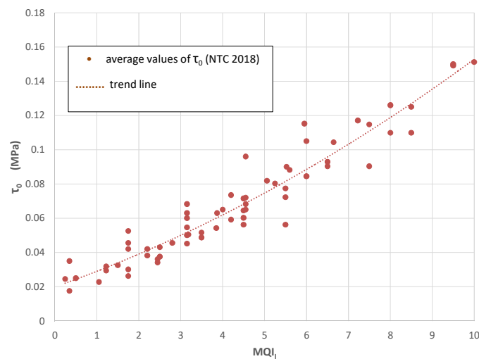
Figure A3. Masonry shear strength \tau_0 vs. MQI_i (NTC 2018, Italian Seismic Code, 2018).
