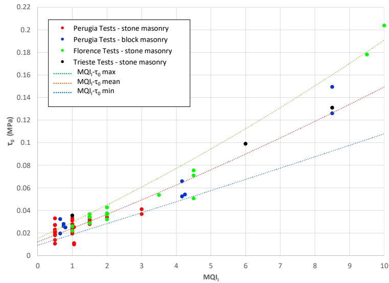
Figure A8. MQI_i vs. shear strength \tau_0 : experimental results are compared with suggested relationships.
