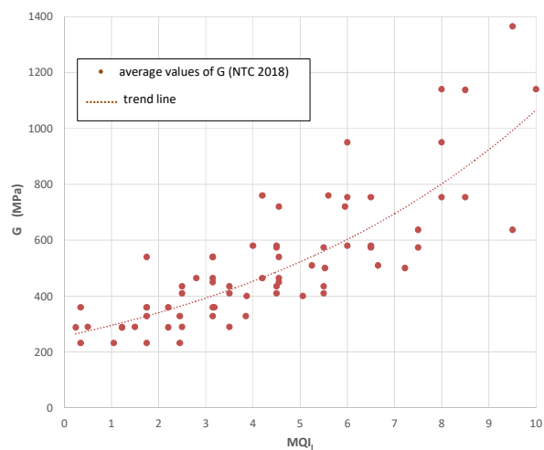
Figure A6. Masonry shear modulus G vs. MQI_i .
