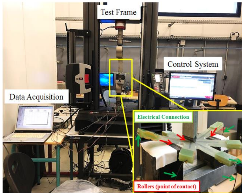
Fig. 5. Setup to examine the in-situ monitoring performance of the Nylon/Ag fiber sensor when integrated with in the composite sample during three-point bend test.
