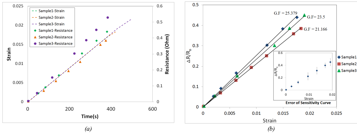
Fig. 6. GF calculation of the Nylon/Ag fiber sensor. (a) shows that all three fiber sensor samples showed good electromechanical response. (b) shows the GF of all three samples with repeatability in results. Error of sensitivity curve was also plotted in this figure of all three samples [63].
