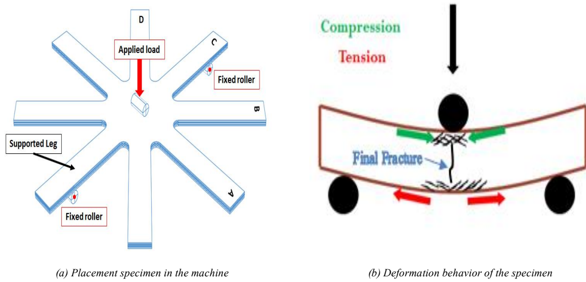
Fig. 7. Deformation behavior of star specimen during three-point bend test.
