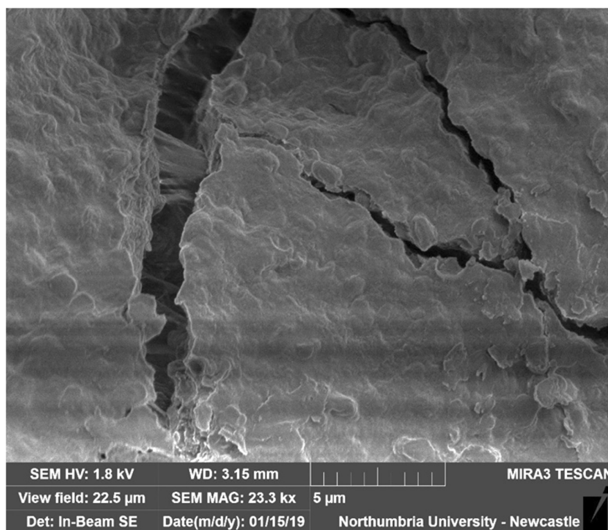
Figure 16. Scanning electron microscopy (SEM) of cracking observed at extreme low relative humidity.
