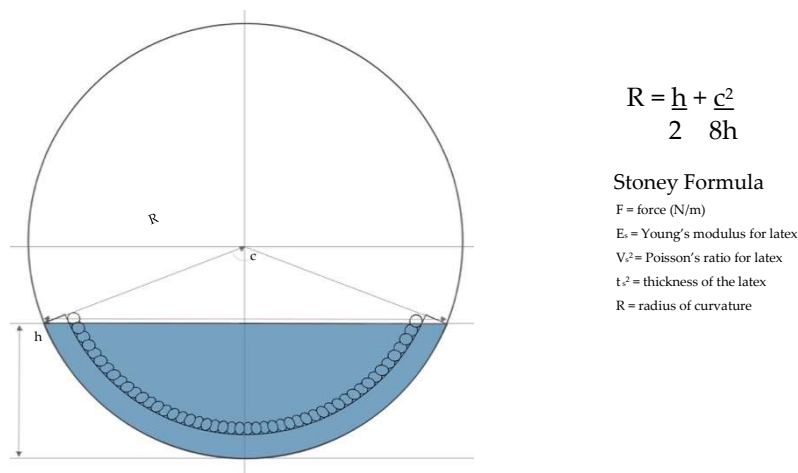
Figure 9. Calculation of force generated by a B. subtilis actuator
