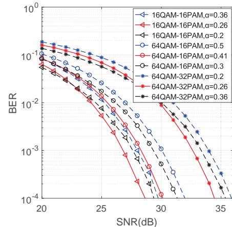
Fig. 3: BER comparisons of the proposed Rx under the different optical power allocations
