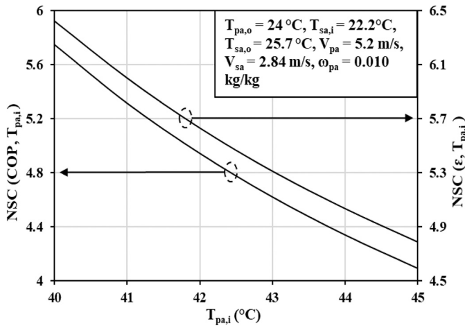
Fig. 14. Variation in NSC of the COP and \epsilon against T_{pa,i} .
