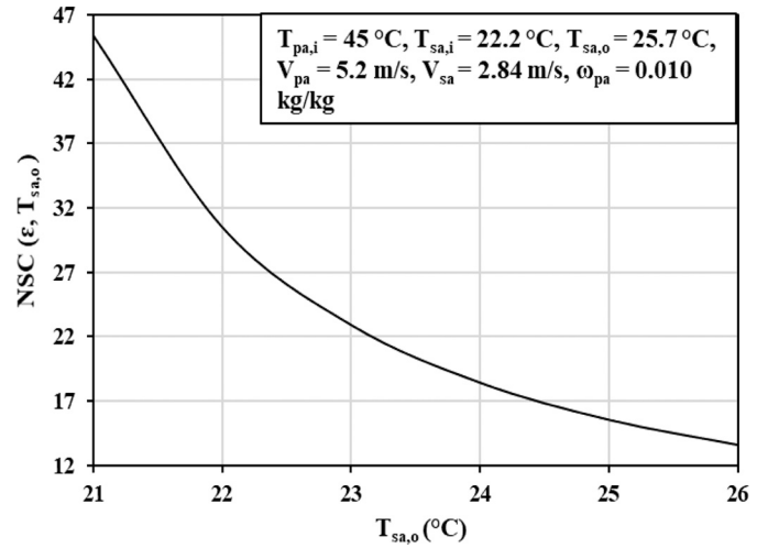
Fig. 17. Variation of NSC of \epsilon against T_{sa,o} .
