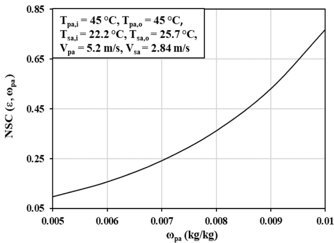
Fig. 16. Variation in NSC of \epsilon against \omega_{pa} .
