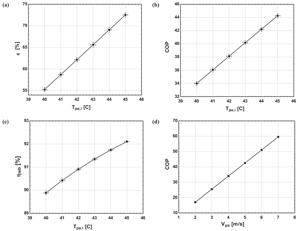
Fig. 13. Uncertainty propagation in (a) \epsilon versus T_{pa,i} , (b) COP versus T_{pa,i} , (c) \eta_{wb} versus T_{pa,i} , and (d) COP versus V_{pa} .
