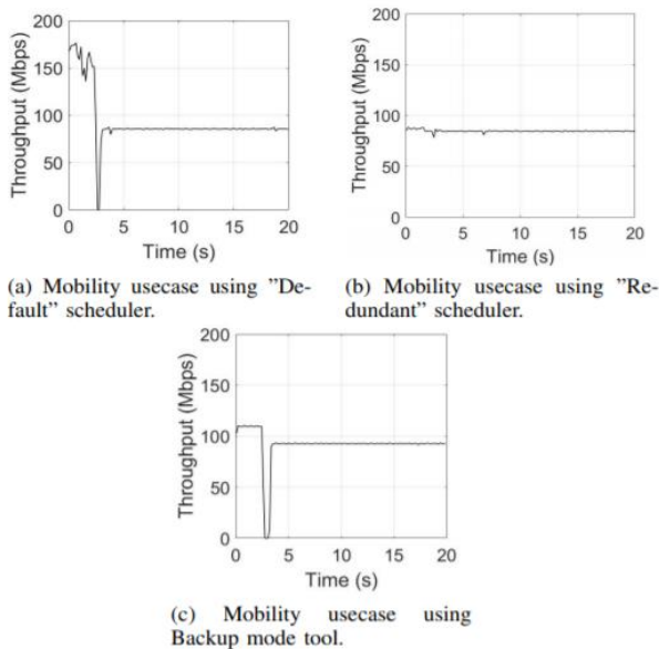
FIG. 5: MPTCP performance in VLC with link blockage due to mobility in "Default", "Redundant" and Backup modes
