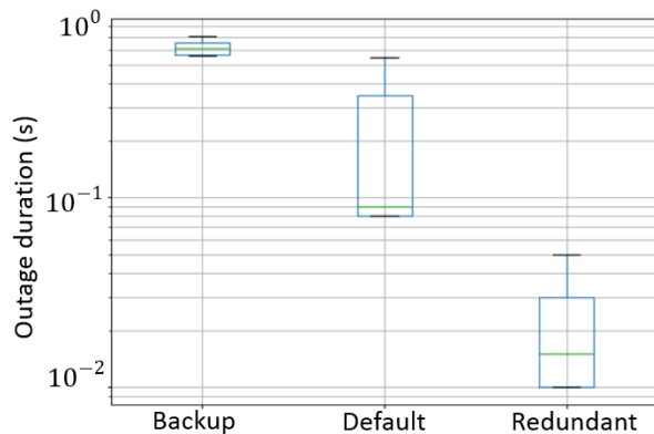
FIG. 7: Outage duration for mobility usecase scenario in a VVLC network.
