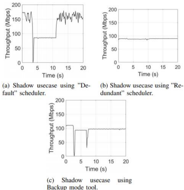
FIG. 6: MPTCP performance in VLC with link blockage due to shadow/obstacle in "Default", "Redundant" and Backup modes.
