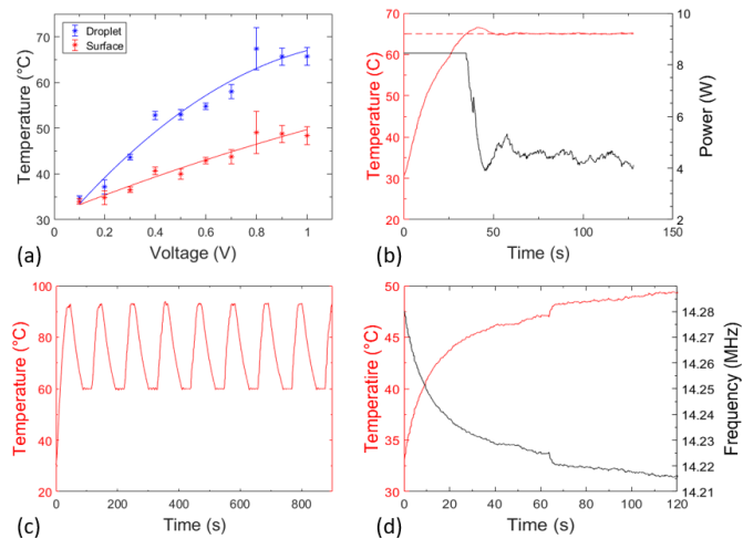
Figure 8 (a) Temperature recordings for droplet and surface using a constant input voltage (peak-to-peak) (b) Example of droplet temperature control (simulated LAMP thermal process); (c) Example of droplet temperature control (simulated PCR thermal cycling), (d) example control of frequency over time
