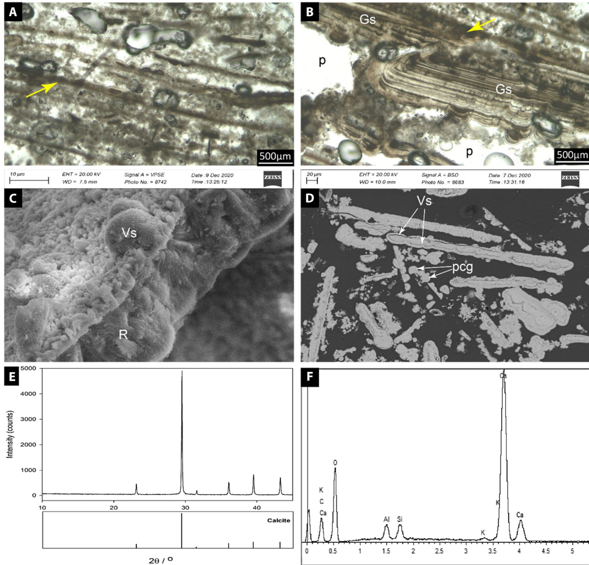
FIGURE 5 FI Coated vegetative remains and carbonate raft (microfacies 1). (A) Assemblage of brown-coloured, flat and elongated vegetative remains (arrow) coated by calcite thin films. (B) Some flat remains (arrow) are covered in globular sparry calcite crusts (Gs); interparticle porosity (p) is very abundant. (C) SEM photomicrograph of carbonate rafts (R) covered by multiple arcuate vault structures (Vs) consisting of cloudy, brown-coloured sparry calcite. (D) BSE-SEM image of poorly sorted carbonate rafts covered by vault structures (VS). Some polycrystalline calcite globular aggregates (pcg) can grow laterally to form elongated structures. (E and F) XRD pattern and EDX spot analysis, respectively, indicating a calcite mineralogy
