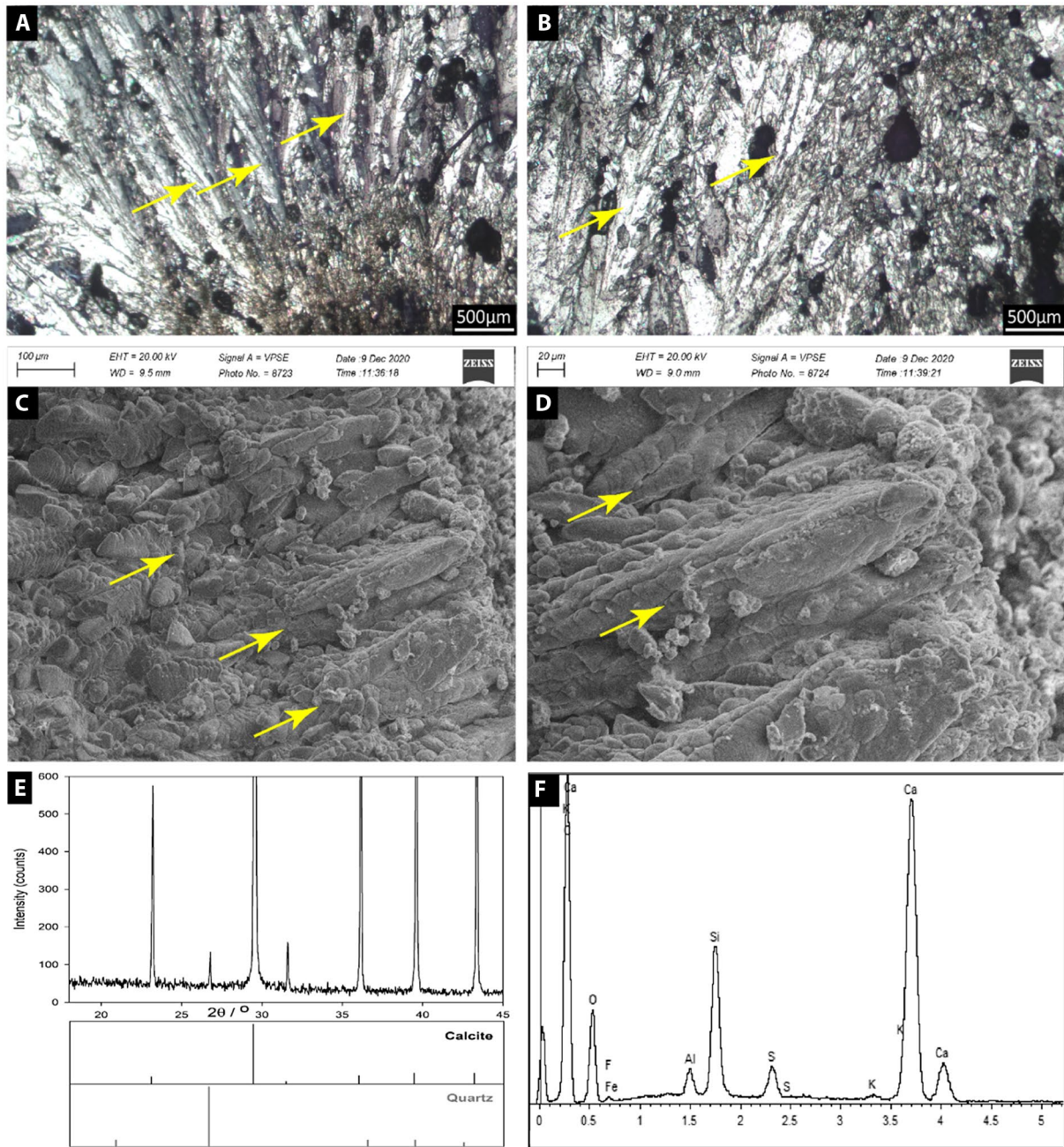
FIGURE 11 Dendrite carbonates (microfacies 7). (A and B) Light grey calcite polycrystals showing multiple levels of branching (arrows). (C and D) BSE-SEM images showing that each branch consists of numerous thin (up to 0.2 mm thick), plate-like calcite crystals that are stacked en echelon (arrows). (E and F) XRD pattern and EDX spot analysis, respectively, indicating that calcite and quartz are present
