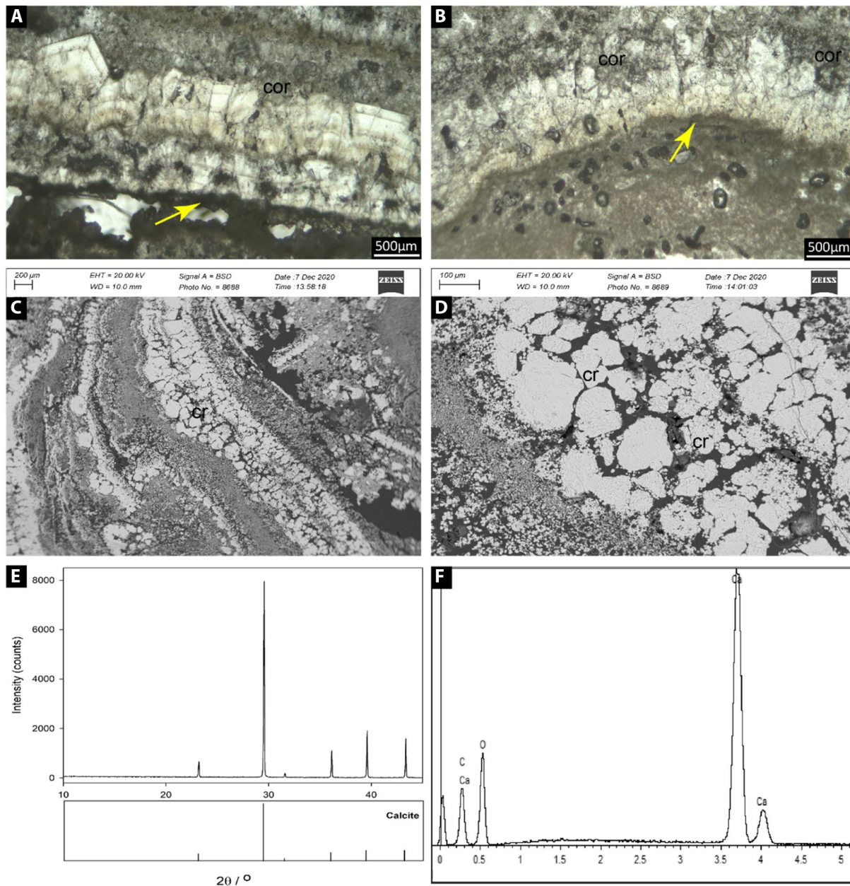
FIGURE 9 Neomorphic sparry crust (microfacies 5). (A and B) Neomorphic sparry crusts growing on top of organic-rich substrates (arrows). Corroded areas (cor) through irregular surfaces on the external part of the crusts are common. (C and D) BSE-SEM images showing cracking of the crusts where fissures (cr) reach different depths showing no apparent reworking. (E and F) XRD pattern and EDX spot analysis, respectively, indicating that calcite is the predominant mineralogy
