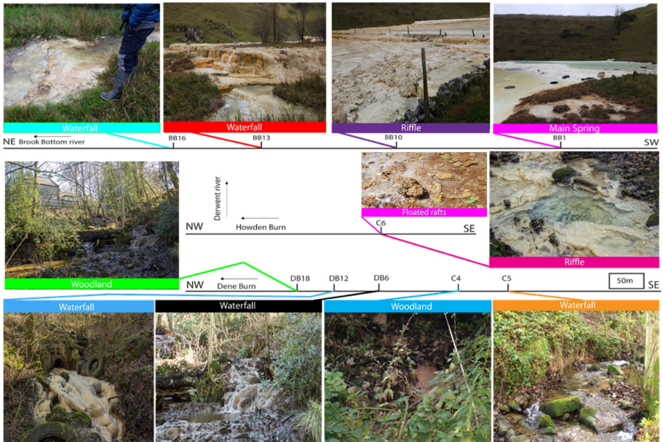
FIGURE 2 Environmental pictures of the downstream transects of Howden Burn, Dene Burn and Brook Bottom with the localisation of the riffle, waterfall and woodland
