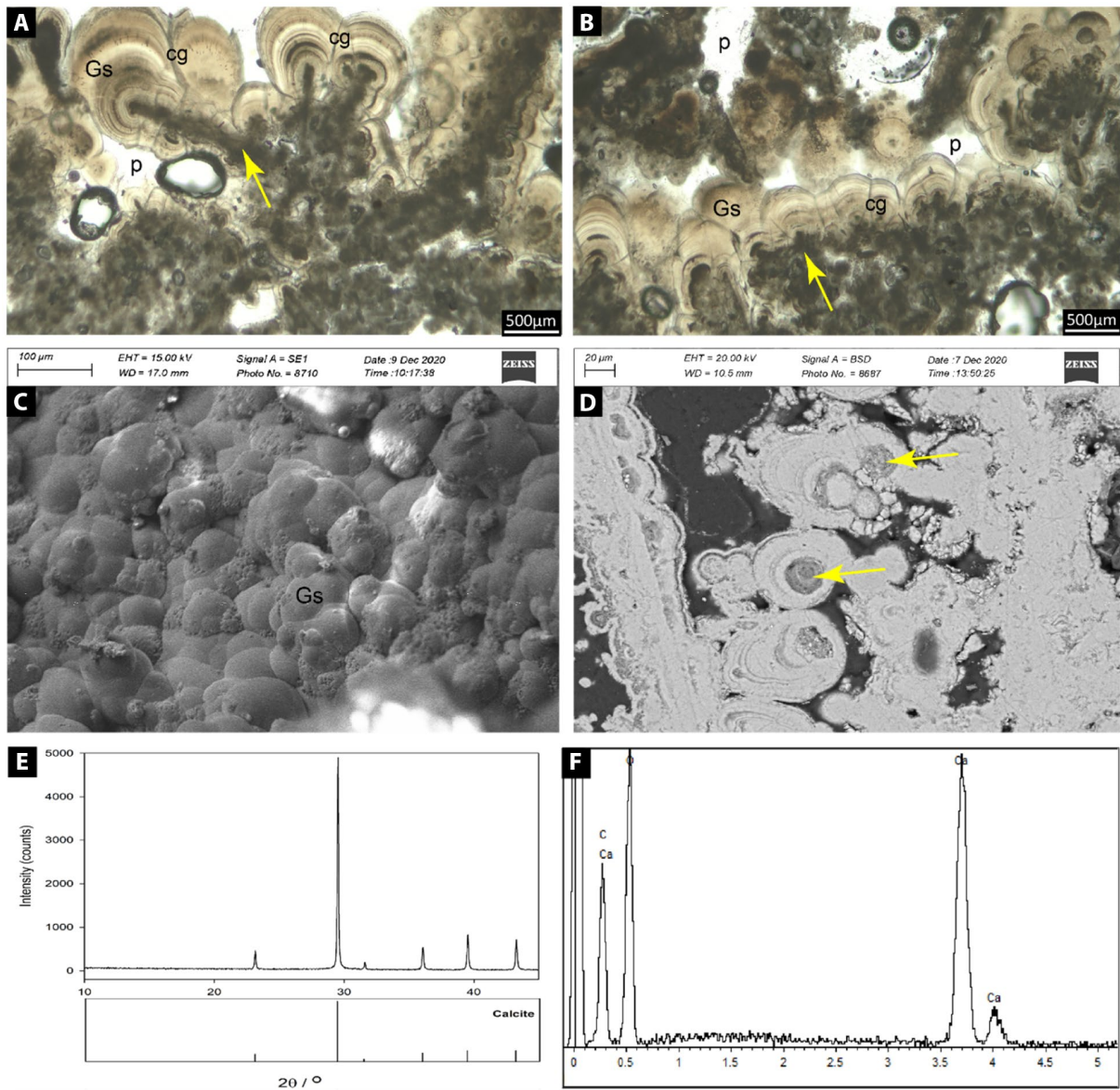
FIGURE 8 Globular sparry calcite crust (microfacies 4). (A and B) Thick isopachous calcite fans with globular arrangements (Gs) growing on top of clotted peloidal templates (arrows). Fans consist of thin darker laminae and thick lighter laminae extending laterally. Competitive growth defines sharp boundaries between fans (cg). This microfacies displays a high intercrystalline porosity (p). (C) SEM image showing the external smooth curved surfaces of the fans (Gs). (D) BSE-SEM image displaying sparry crusts growing on top of organic substrates (arrows). Note thin concentric, darker laminae within fans. (E and F) XRD pattern and EDX spot analysis, respectively, indicating that calcite is the predominant mineralogy
