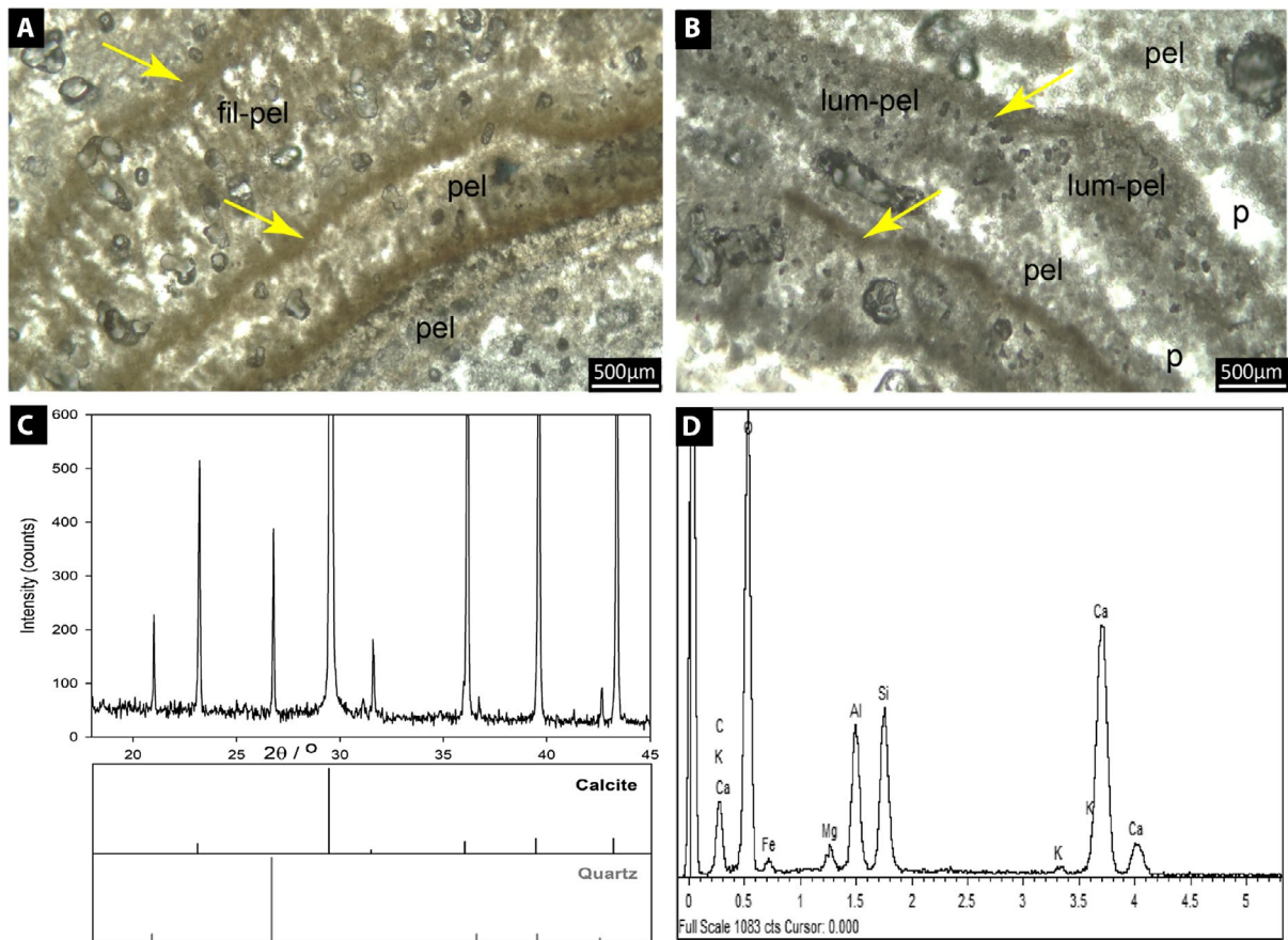
FIGURE 6 Micropeloidal and clotted micritic (microfacies 2). (A and B) Patchy micropeloidal micritic textures (pel) alternate with laminated textures (arrows). Filamentous clotted structures can be seen perpendicular to laminae (fil-pel). In some cases, lumpy micropeloidal masses (lum-pel) develop in association with laminated textures. Abundant intercrystalline porosity (p) is observed in this microfacies. ++(C and D) SEM images of the microfacies clotted micrite. XRD pattern and EDX spot analysis, respectively, indicating that calcite and quartz are present
