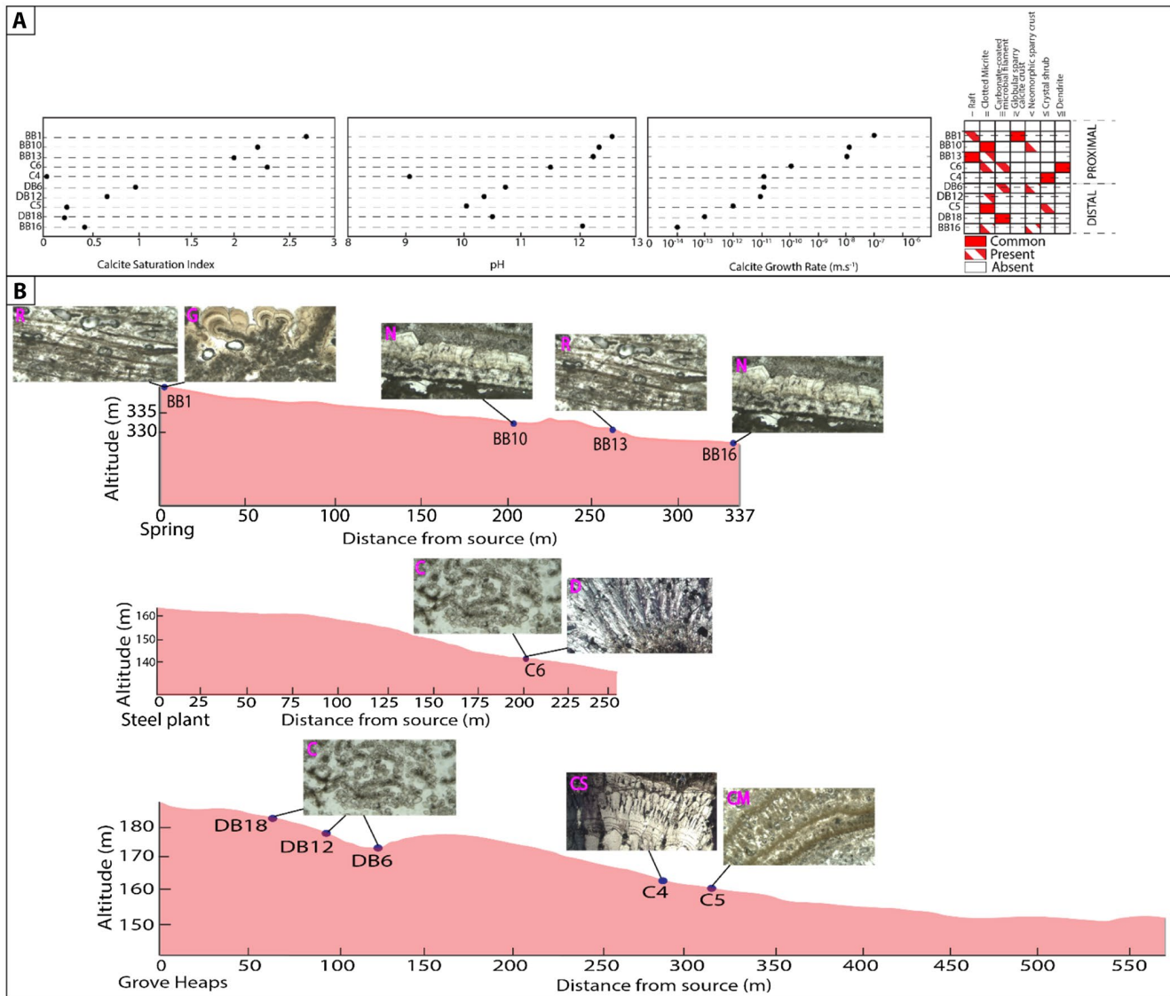
FIGURE 14 (A) Diagram showing the Calcite Saturation Index (CSI), pH, calcite growth rate (R) versus distribution of microfacies according to the sample locations at Brook Bottom (BB) BB1, BB13, BB10 fresh, BB10 old deposit, BB16 and Consett (C) freshwater samples in Howden Burn (C6) and Dene Burn (DB) (C4, C5, DB6, DB12, DB18). (B) Depositional model summarising the lateral changes of the dominant microfacies: Coated vegetative remains and carbonate raft (R), Micropeloidal and clotted micritic (CM), Carbonate-coated microbial filament (C), Globular sparry calcite crust (G), Neomorphitic sparry crust (N), Crystal shrub (CS) and Dendrite (D)
