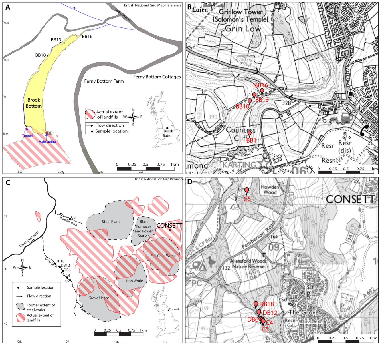
FIGURE 1 (A) Location map of the Brook Bottom (BB) samples (BB1, BB13, BB10 fresh, BB10 old deposit, BB16) where the yellow part represents the carbonate deposit. (B) Topographic map with the Brook Bottom samples (BB1, BB13, BB10 fresh, BB10 old deposit, BB16) after Ordnance Survey map. (C) Location map of the Consett (C) freshwater samples in Howden Burn (C6) and Dene Burn (DB) (C4, C5, DB6, DB12, DB18) after Historic OS maps. (D) Topographic map with the Consett freshwater samples in Howden Burn (C6) and Dene Burn (C4, C5, DB6, DB12, DB18) after Ordnance Survey map
