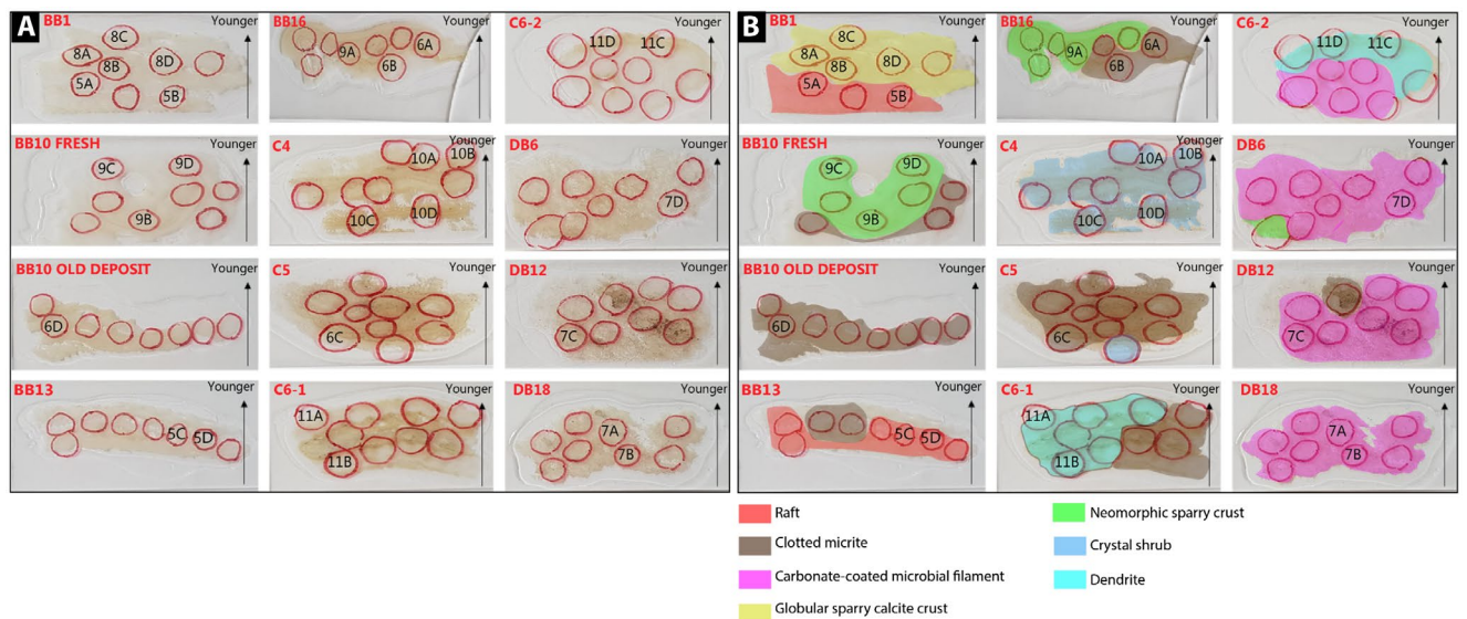
FIGURE 3 (A) Original thin sections from the Brook Bottom (BB) (BB1, BB13, BB10 fresh, BB10 old deposit, BB16) and Consett (C) freshwater samples in Howden Burn (C6) and Dene Burn (DB) (C4, C5, DB6, DB12, DB18) with the locations of the optical microscope images. The locations are respectively designated by the number of the figure from this manuscript followed by the letter corresponding to the subsection in the figure. (B) Interpreted thin sections with the colours representing the different microfacies. The locations of the optical microscope images are respectively designated by the number of the figure from this manuscript followed by the letter corresponding to the subsection in the figure
