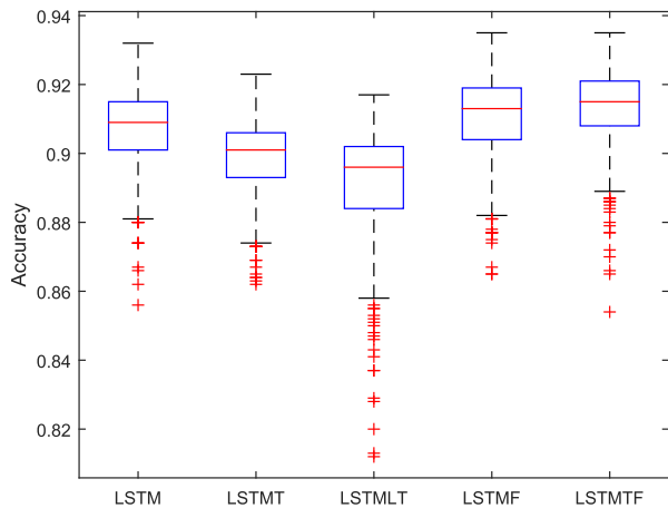
Fig. 3 Stability of five models on the test set
