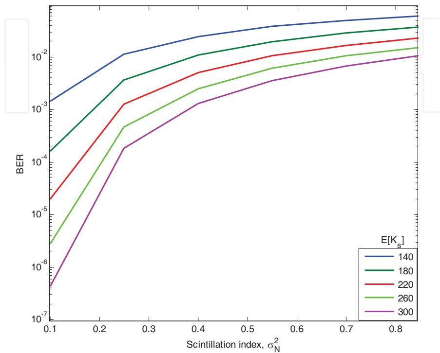
Fig. 15. Binary PPM BER as a function of scintillation index for K_{Bg} = 10 ; T_e = 300 K, \zeta = 0.028 , R_b = 155 Mbps and \bar{g} = 150 .
