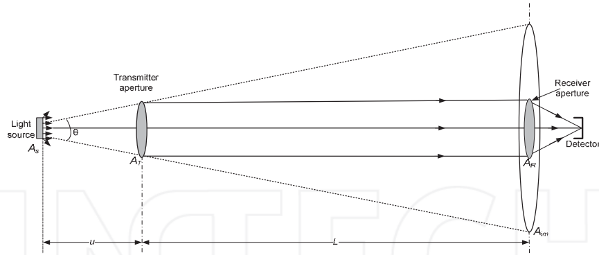
Fig. 7. Beam divergence
