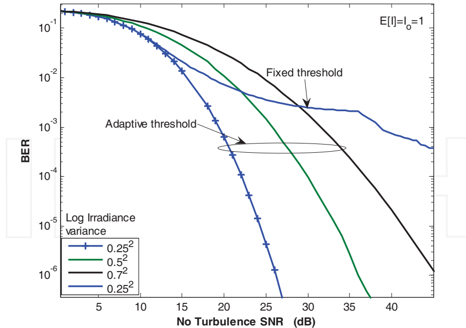
Fig. 13. BER against the SNR for fixed and adaptive thresholds and various levels of scintillation.
