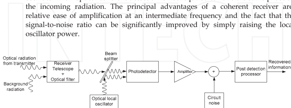
Fig. 5. The block diagram of a coherent detection optical receiver.
