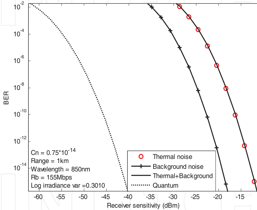
Fig. 17. The BER against the receiver sensitivity under different noise sources, with R_b = 155 Mbps, \sigma_l^2 = 0.3 and \xi = 1 .
