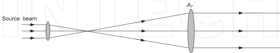
Fig. 8. Beam expander diagram
