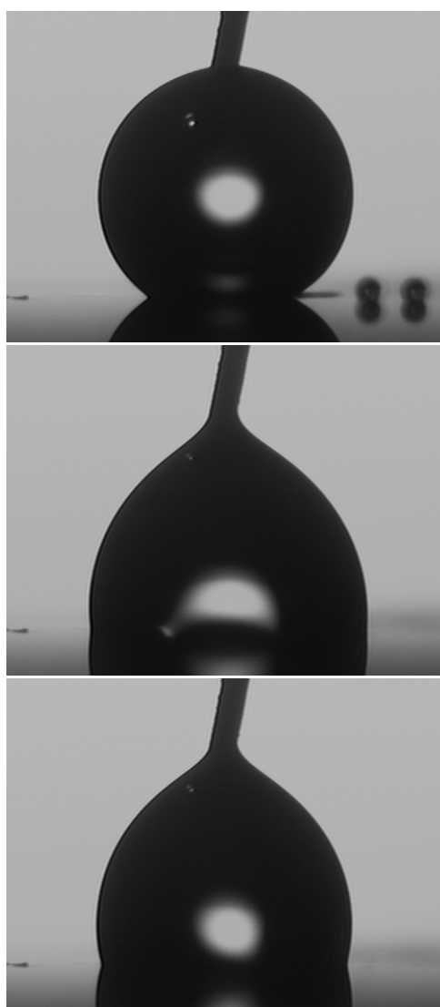
Fig. 2. Image of a water drops on a SU-8 patterned surface with a Teflon ® AF overlayer showing the Initial drop (upper), drop with maximum applied voltage (centre) and drop with voltage removed (lower).
