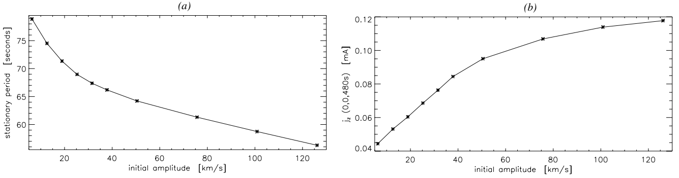
Fig. 4. a) Stationary period, i.e. the time taken to evolve from the second horizontal current sheet to the third (measured in seconds) and b) j_{\text{final}} , i.e. j_z(0, 0) evaluated at t = 480 s, (measured in milliAmps) versus initial velocity amplitude (measured in \text{km s}^{-1} ), where v_0 = 25.2 \text{ km s}^{-1} corresponds to C = 1 simulation.
