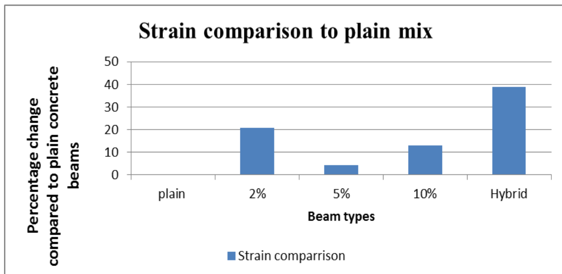
Figure 2 – Strain comparison
