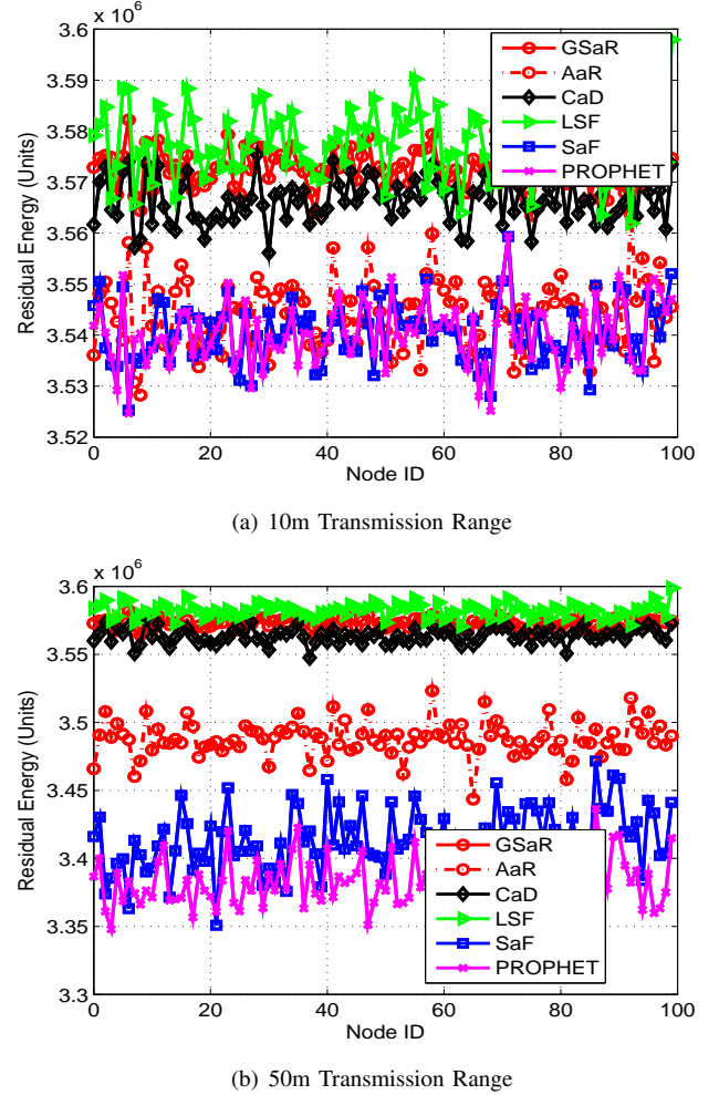
Fig. 12. Energy Distribution
