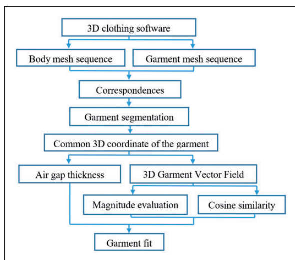
Figure 1. Overview of the method: (a) 3D clothing software is first used to simulate the dynamic garment and to export (b) the body mesh sequence, and (c) the garment mesh sequence; (d) the correspondences between the garment and the body are automatically calculated; (e) the garment is automatically segmented; (f) a new method is proposed to build a common 3D coordinate for the garments in frames; (g) based on (f), the dynamic air gap thickness is determined, and (h) the 3D garment vector field (3DGVF) is presented to represent the garment sliding. (i) Magnitude evaluation and (j) cosine similarity are used to evaluate the directional and scalar changes of 3DGVF; and (k) the indicator values are compared to explore the fit.
