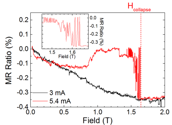
FIG. 6. MR of an Ortho-NC-STO measured below ( I=3 mA; black curve) and above ( I=5.4 mA; red curve) threshold. Above threshold, the droplet is fully formed at about 1 T. As the OOP field is further increased, the droplet becomes unstable and finally collapses at about 1.64 T.
