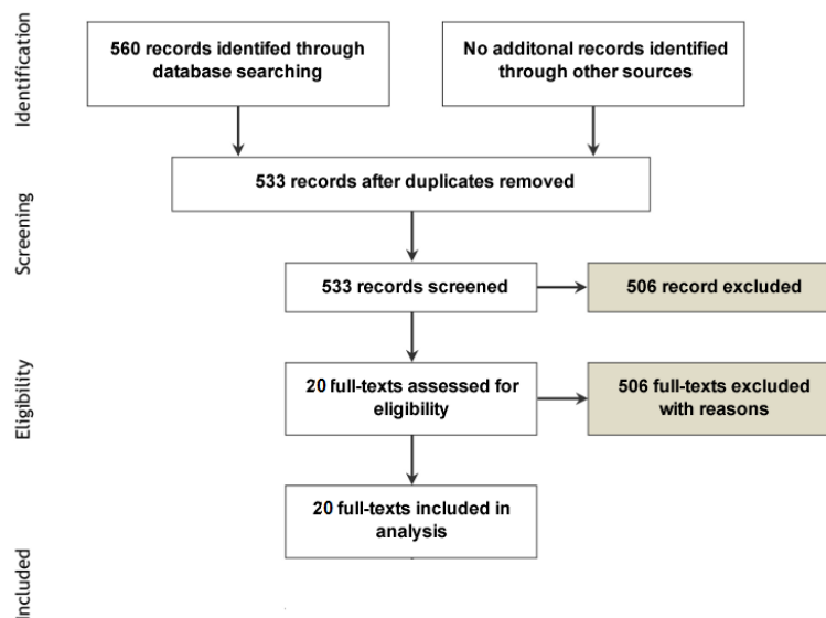
Figure 1: SLR process
