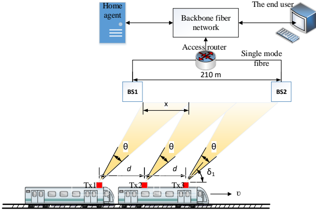
Fig. 4 Train to ground communication where the coverage area of each transceiver is 75m. The transceivers are spaced 75m apart from each other.
