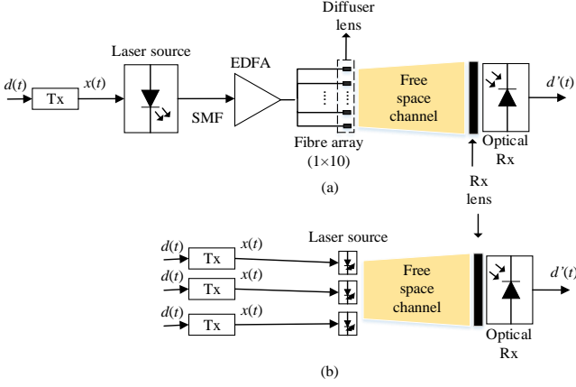
Fig. 1 A block diagram of line of sight FSO transmission for: (a) from ground-BS to the train and (b) from train to the ground-BS
