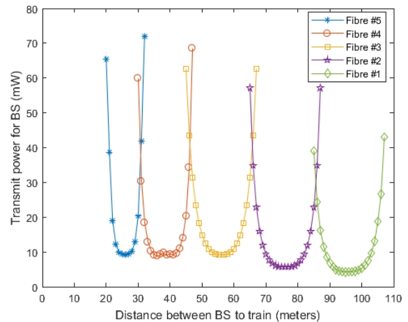
Fig. 10 The transmit power as a function of transmission distance for laser/fibre 1-5
