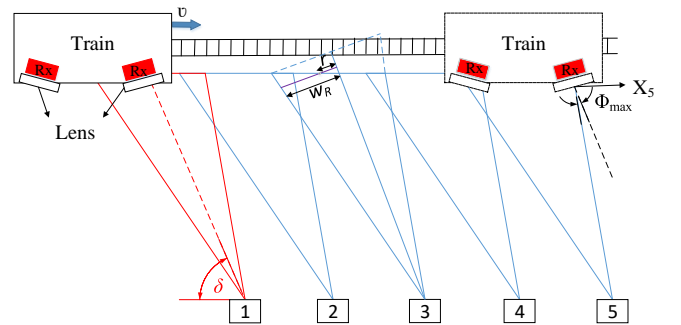
Fig. 3 The Rx's alignment offset angle with respect to the transmit beam (1-5) direction.
