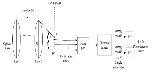
Fig. 6 The Rx configuration based on series of cascading lenses
