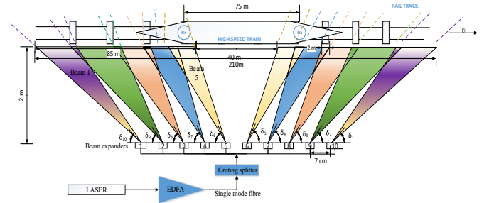
Fig. 2 The laser/fibre array covers 170 m (85 m on either side). The distance between the two BSs is 210 m.
