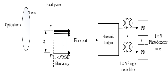
Fig. 8 Schematic block diagram of a single lens setup
