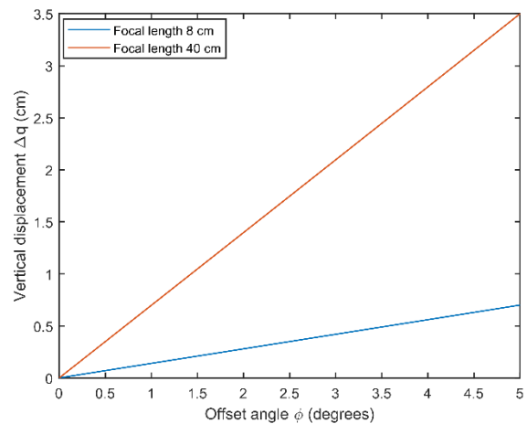
Fig. 7 Vertical displacement as a function of the offset angle for f of 8 and 40 cm.
