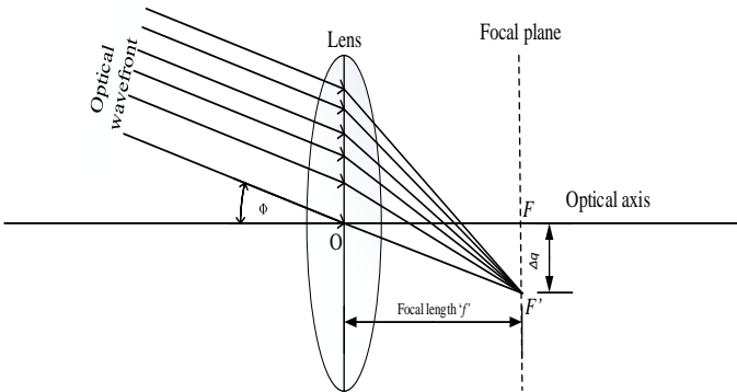
Fig. 5 Oblique beam through a perfect lens
