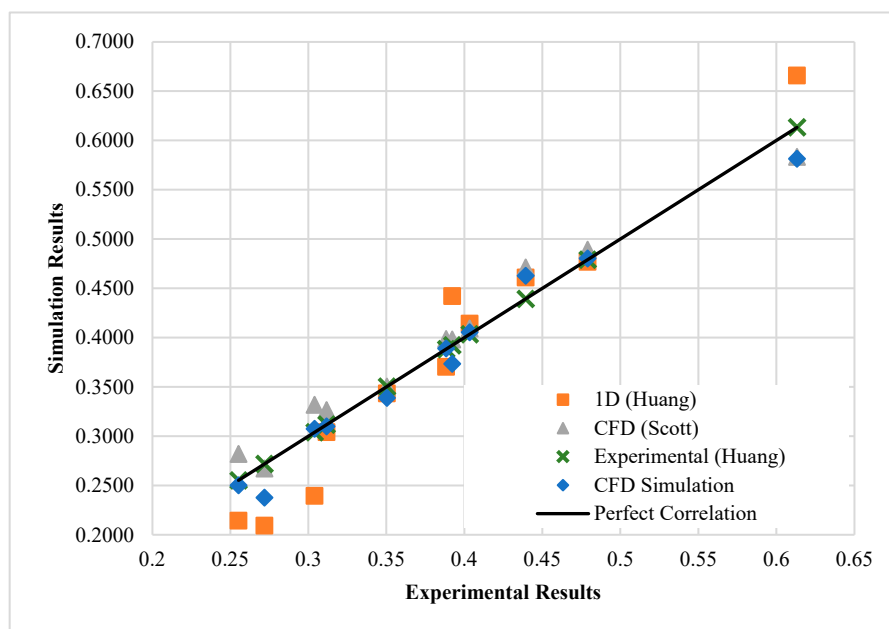
Figure 9. Validation of CFD modeling with published data.
