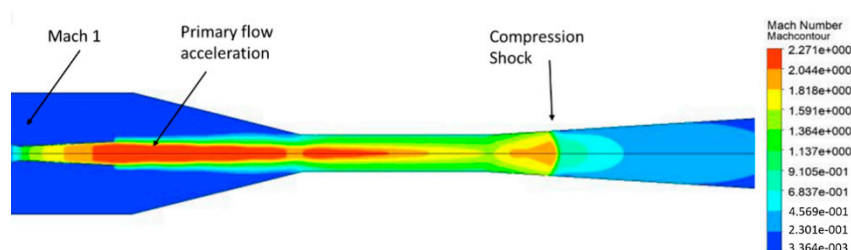
Figure 6. CFD results and validation: Mach contours with R141b working fluid for model from [25,34].
