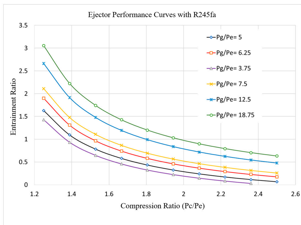
Figure 14. R245fa-Performance curves for Ejector.
