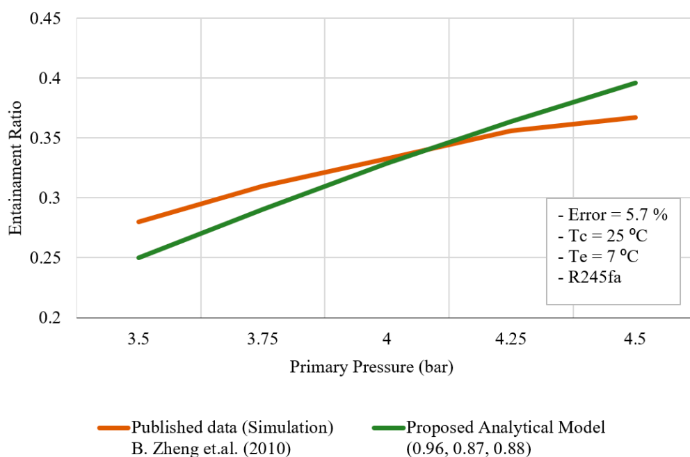
Figure 13. Validation with simulation data from literature.
