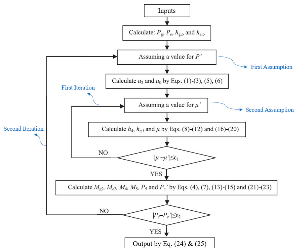
Figure A3. Computation procedure used by Chen [40] for their 0-D model.
