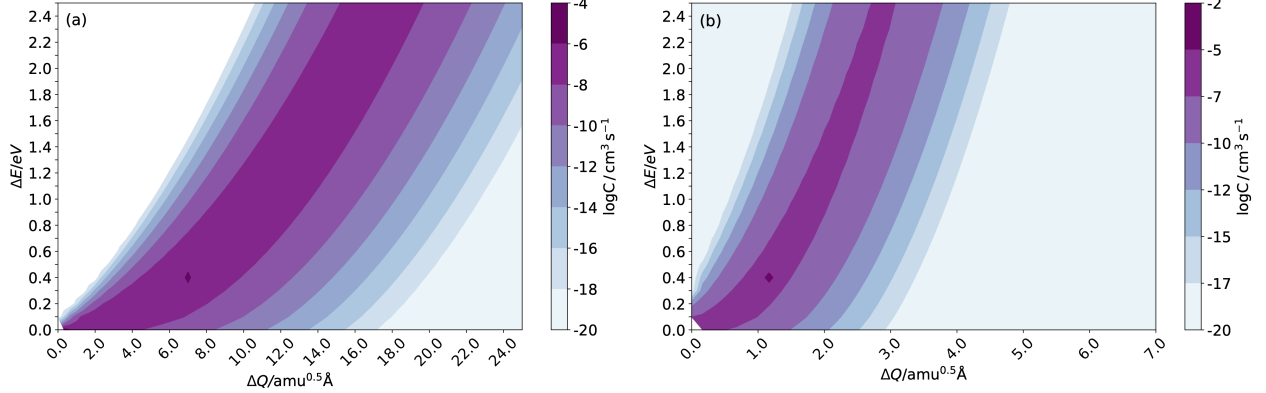
Figure 2: Variation of the carrier capture coefficient C with the parameters \Delta E and \Delta Q using Equation 2. This data is for the single frequency approximation and taking frequencies near the extrema of the physical range: (a) \hbar\omega = 8 meV and (b) \hbar\omega = 50 meV.
