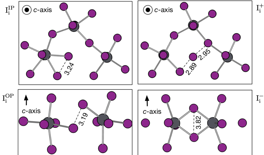
Figure 3: Defect geometries of I_1^+ , I_1^- , I_1^{IP} and I_1^{OP} in CH_3NH_3PbI_3 . IP indicates that the neutral defect is lying in the ab -plane. OP indicates that the defect is lying along the c -axis. All distances are measured in units of Å. The iodine is coloured in purple and the lead in grey. For clarity, the organic cations are not show.
