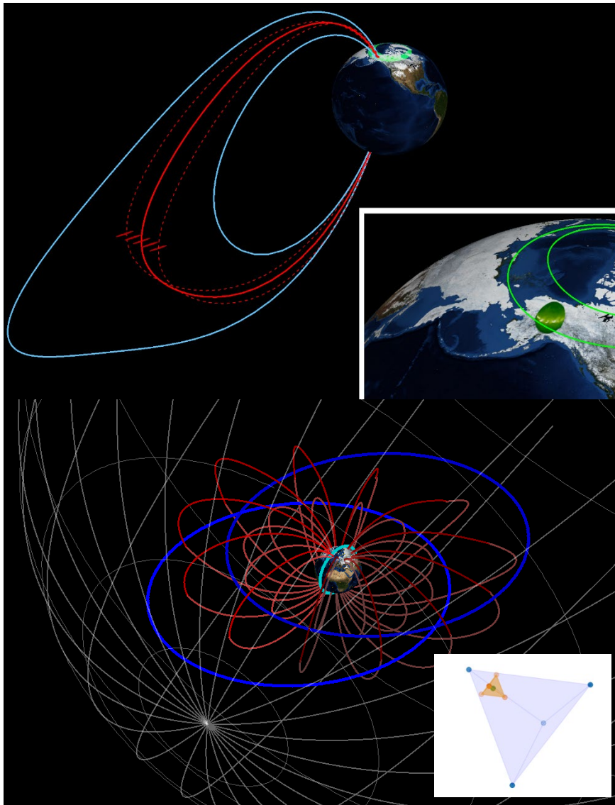
Figure 8. (top) Studying kinetic plasma physics in the region of explosive energy release during a terrestrial substorm (inset). The nested tetrahedral are shown with an active experiment in green in the smallest tetrahedral to study the physics of M-I coupling.
