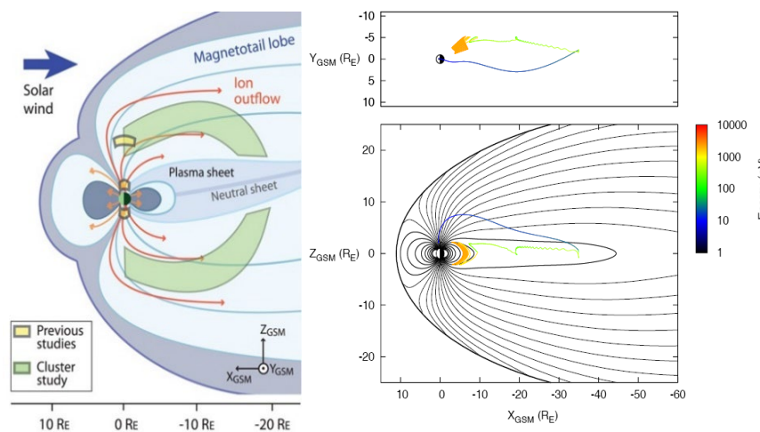
Figure 6. Left: Schematic of “cold hidden” H + ion outflow in the magnetosphere, regions of existing satellite observations (adapted from Engwall et al., 2009); right: Typical trajectory of an O + ion originating from the cleft ionosphere as it transits the magnetosphere (after Howarth and Yau 2008)
