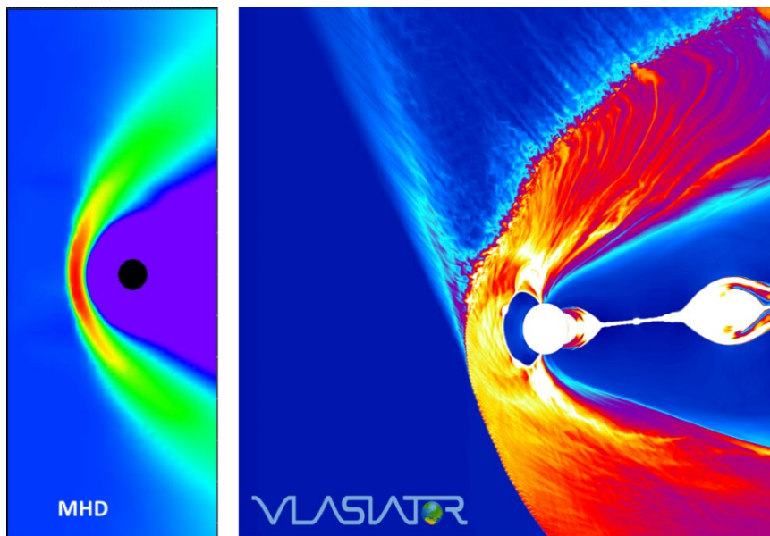
Figure 1. Global magnetospheric simulations on (left) MHD fluid scales, and (right) hybrid kinetic-ion scales highlighting the complexity of solar wind-magnetosphere interaction across kinetic scales (M. Palmroth and Vlasiator team; Palmroth et al., 2018)
