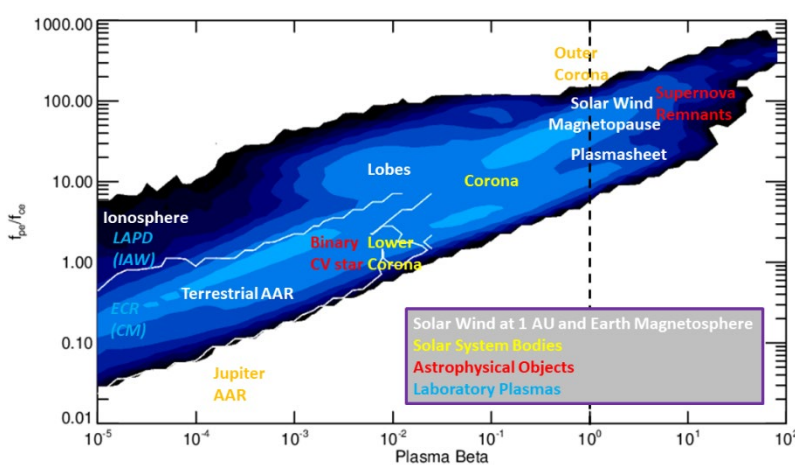
Figure 4. Properties of various Solar System, astrophysical objects, and lab plasma regimes as a function of plasma frequency ( f_{pe} ), electron gyrofrequency ( f_{ce} ), and plasma beta ( \beta ). In colour are real measurements from the Cluster spacecraft over the mission lifetime, superimposed on this are regimes of each Solar System, lab plasma, or astrophysical object.
