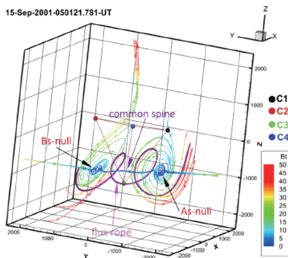
Figure 3. Magnetic field reconstruction results for a flux rope event showing a separator connecting a pair of A-B null points (after, Guo et al., 2013) and the limitation of a small spacecraft array for multiple structure.
