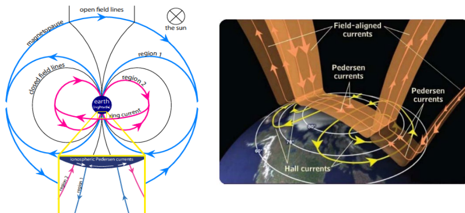
Figure 5: Magnetospheric current systems, linked via field-aligned currents (left) Coxon et al. (2014) and (right) COMET program, UCAR 7
