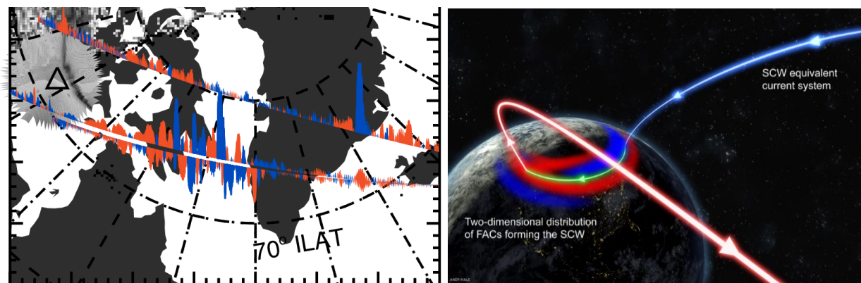
Figure 5. (left) Cluster observations of the spatial scales of FACs in the nightside magnetosphere-ionosphere; blue denoting FACs directed towards the ionosphere and red denoting FACs directed away from the ionosphere, together with (right) a schematic representation of the FAC structure on fluid scales. Left: adapted from Forsyth et al. (2014); right: Murphy et al. (2013)
