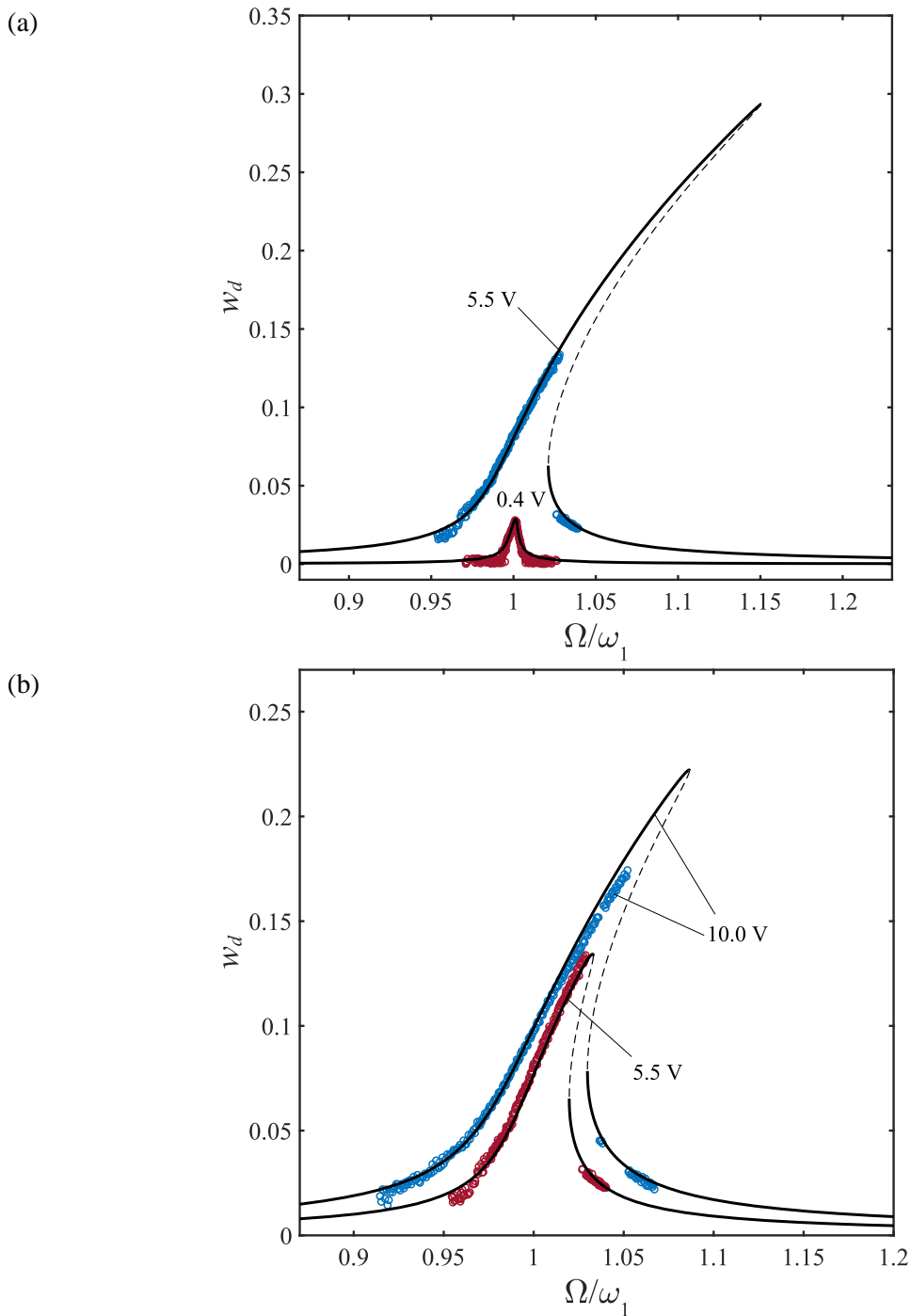
Fig. 3. Frequency responses of the MEMS resonator at V_{DC} = 5 V, and different AC voltages (denoted on the curves). Circles: experimental data; lines: theoretical predictions using the Kelvin-Voigt model with a coefficient of (a) \eta_d = 2.10 \times 10^{-4} calibrated based on the experimental results for V_{AC} = 0.4 V and (b) \eta_d = 5.80 \times 10^{-4} calibrated based on the experimental results for V_{AC} = 5.5 V.
