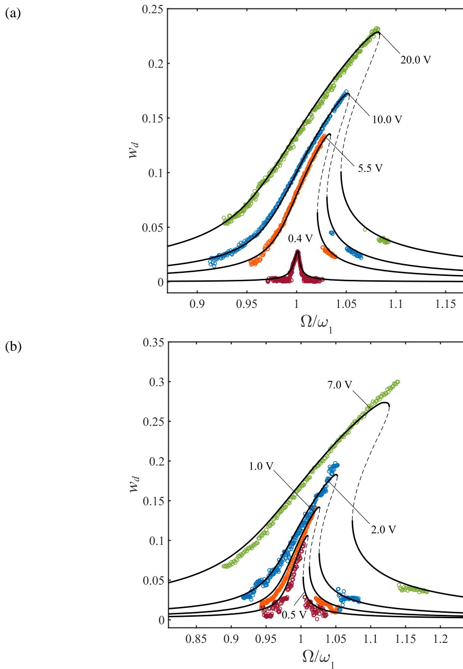
Fig. 6. Frequency responses of the MEMS resonator at (a) V_{DC} = 5 V and (b) V_{DC} = 30 V, and various AC voltages (denoted on the curves). Circles: experimental data; lines: theoretical predictions using the cubic damping model with the two damping coefficients calibrated based on the experimental data for V_{AC} = 0.4 and 5.5 V (sub-figure (a)).
