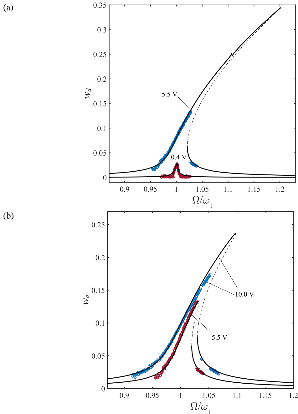
Fig. 2. Frequency responses of the MEMS resonator at V_{DC} = 5 V, and different AC voltages (denoted on the curves). Circles: experimental data; lines: theoretical predictions using the linear damping model with a coefficient of (a) c_d^{(1)} = 0.107 calibrated based on the experimental results for V_{AC} = 0.4 V and (b) c_d^{(1)} = 0.305 calibrated based on the experimental results for V_{AC} = 5.5 V.
