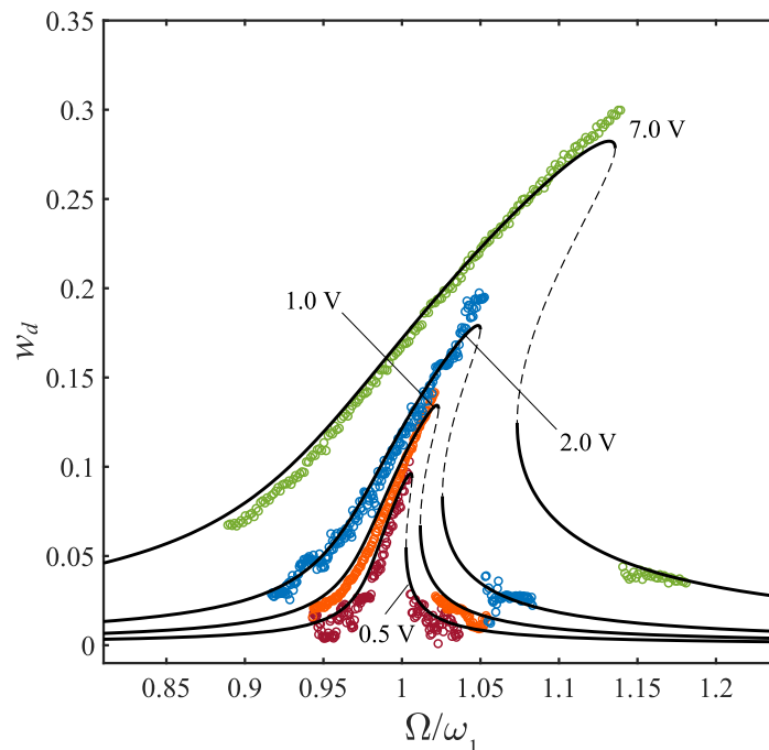
Fig. 5. Frequency responses of the MEMS resonator at V_{DC} = 30 V, and for various AC voltages (denoted on the curves). Circles: experimental data; lines: theoretical predictions using the modified Kelvin-Voigt model with the same damping coefficients as the ones used in Fig. 4.
