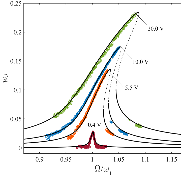
Fig. 4. Frequency responses of the MEMS resonator at V_{DC} = 5 V, and various AC voltages (denoted on the curves). Circles: experimental data; lines: theoretical predictions using the modified Kelvin-Voigt model with the two damping coefficients calibrated based on the experimental data for V_{AC} = 0.4 and 5.5 V.
