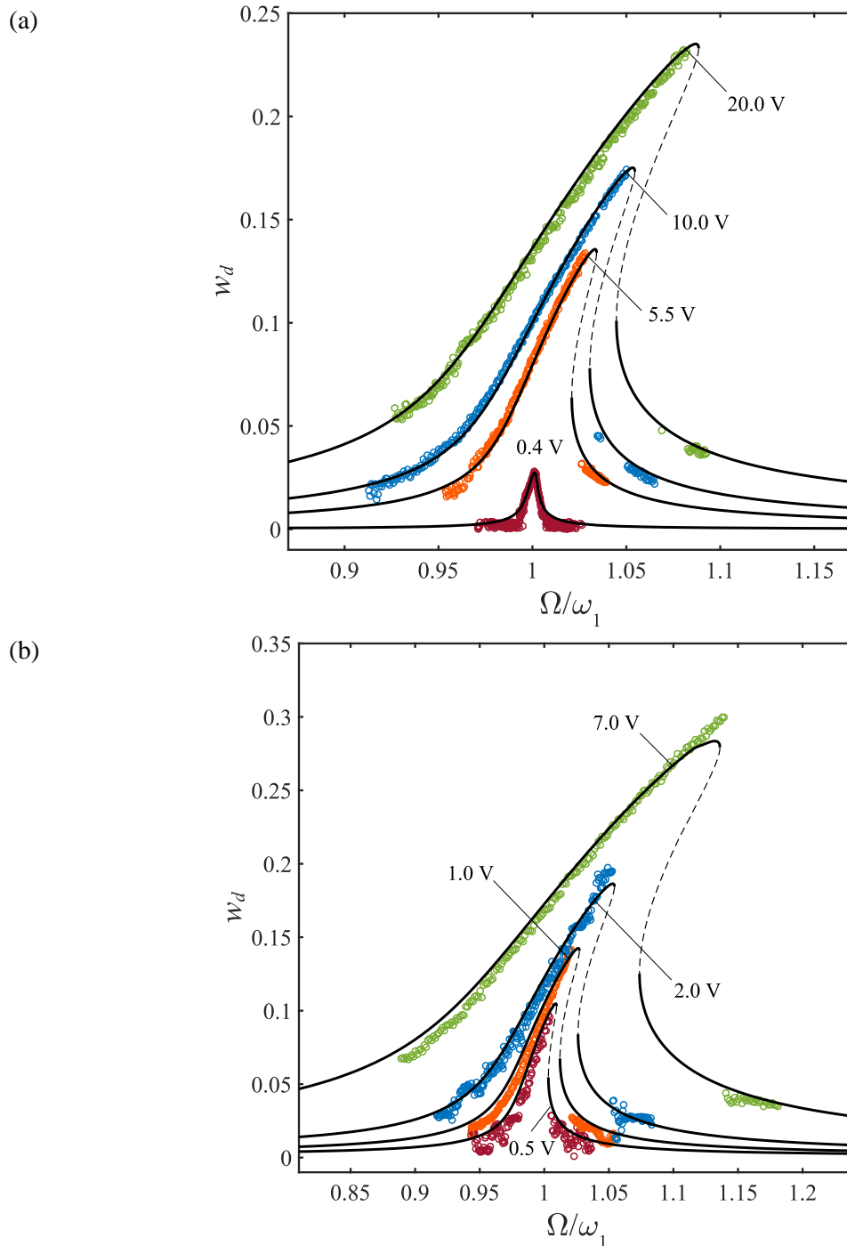
Fig. 7. Frequency responses of the MEMS resonator at (a) V_{DC} = 5 V and (b) V_{DC} = 30 V, and various AC voltages (denoted on the curves). Circles: experimental data; lines: theoretical predictions using the general quadratic-cubic damping model with the three damping coefficients calibrated based on the experimental data for V_{AC} = 0.4, 5.5, and 10 V (sub-figure (a)).
