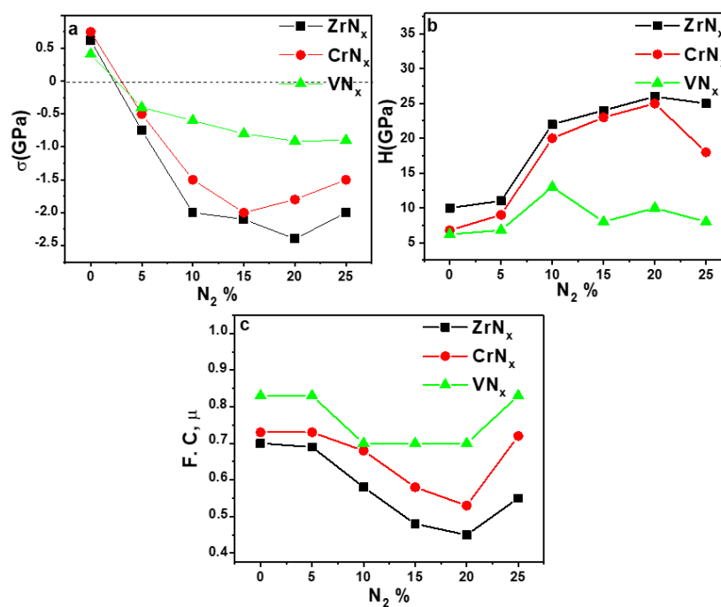
Figure 8. Variation of: (a) residual stress ( \sigma ), (b) hardness (H), and (c) friction coefficient as a function of nitrogen percentage Reprinted from Refs. [16,17].
