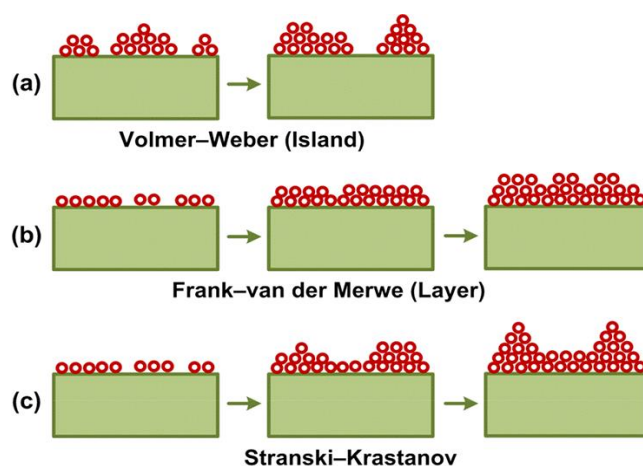
Figure 5. Illustration of (a) Volmer-Weber, (b) Frank-Van Der Merwe, and (c) Stranski-Krastanov thin film and coatings growth modes on substrate surface Reprinted from Ref. [30].
