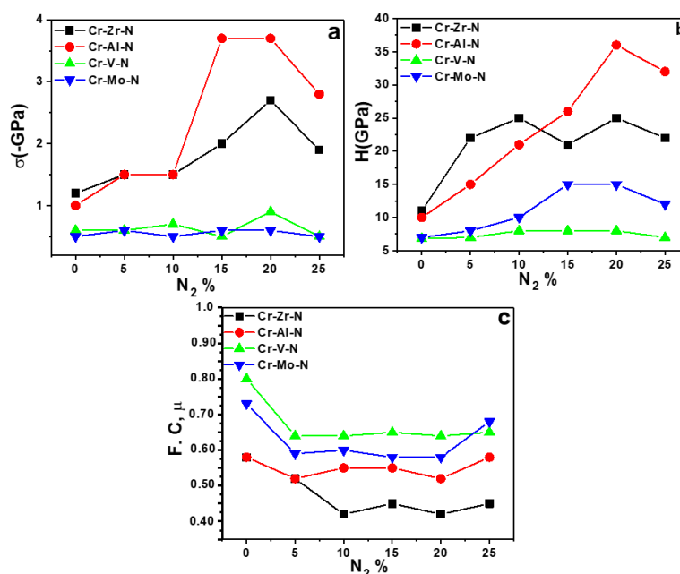
Figure 11. Variation of (a) residual stress ( \sigma ), (b) hardness (H), and (c) friction coefficient ( \mu ) as a function of nitrogen percentage of ternary chromium nitride films Reprinted from Refs. [12,48,49].
