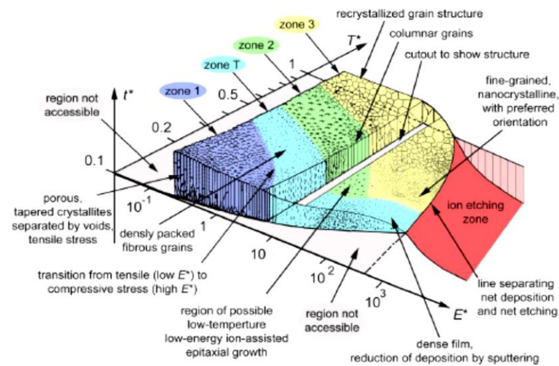
Figure 6. Anders's model of the film structure zone diagram Reprinted from Ref. [31].
