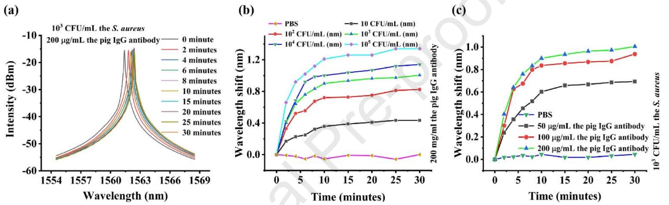
Fig. 5: (a) Spectral responses of the SCS-based EDFL biosensors treated with 200 \mu\text{g}/\text{mL} porcine IgG antibody for detecting 10^3 CFU/mL S. aureus solution concentration, (b) measured wavelength change at different concentrations of S. aureus samples ( 10 , 10^2 , 10^3 , 10^4 , and 10^5 CFU/mL), and (c) different IgG antibody concentrations (50, 100, and 200 \mu\text{g}/\text{mL} ) for detecting S. aureus .
