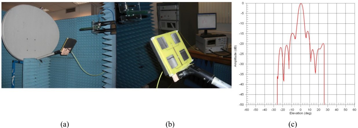
Fig. 2. (a) The overall view of the reflector antenna fed by solar patch (b) Solar patch feed antenna (c) Measured radiation pattern
