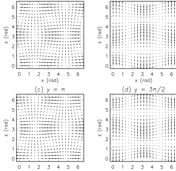
Figure 4. Vector plot of B on (x, z) plane for solution with A_{111} = l = m = n = 1 . The same data as in Fig. 3 is used.
