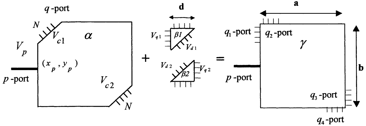
Figure 9.3.1: Microstrip fed antenna and desegmentation method
