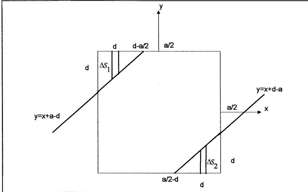
Figure 4C.1 . The unperturbed square patch antenna
