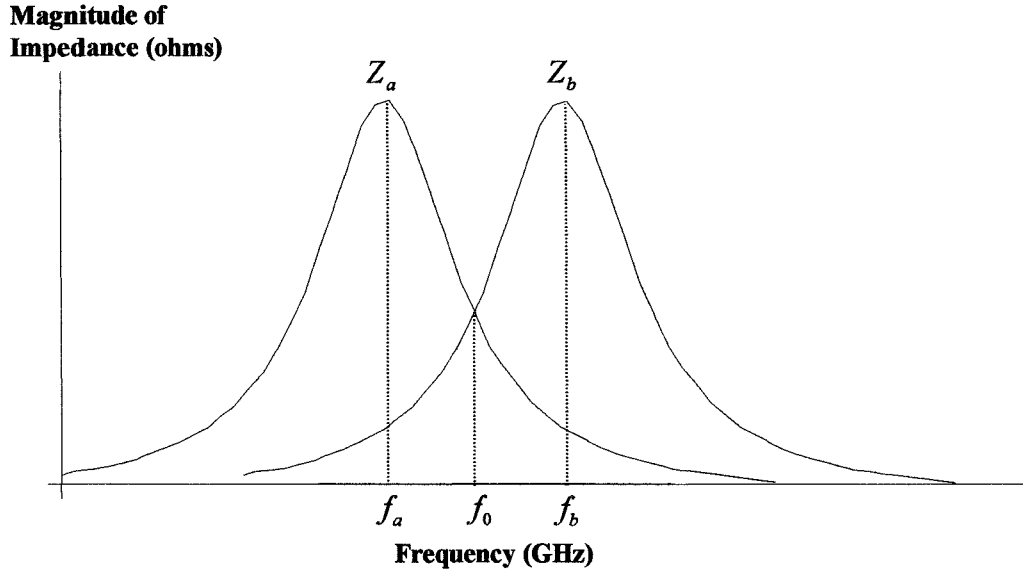
Figure 4.4.2: Two mode resonant frequencies
