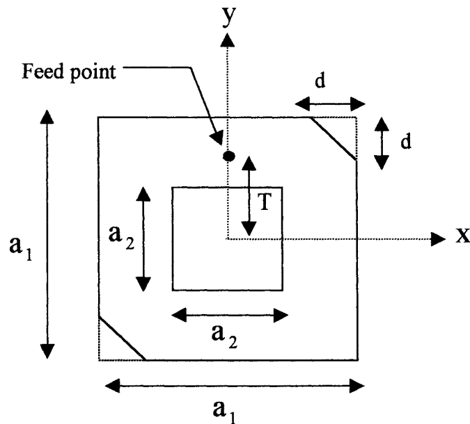
Figure 10.2.1: Square ring microstrip antenna with truncated corners
