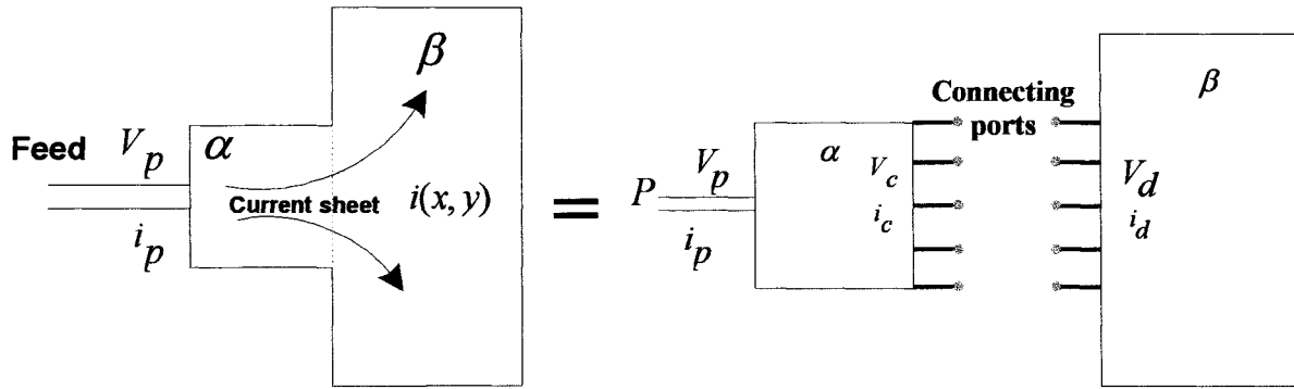
Figure 6.1.1: Current sheet on antenna
