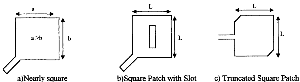
Figure 3.4.3: Single Feed Circularly Polarised Microstrip Patch Antennas
