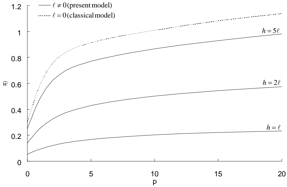
Fig. 7. Effect of the power law index p on the deflection \bar{w} of a square plate
