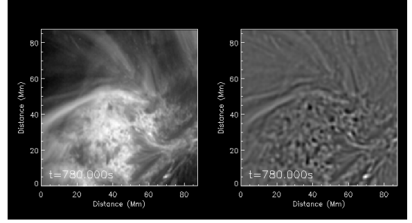
Fig. A.3. Still from Movie 2. The movie shows the same coronal structure as that in Movie 1 as observed with SDO/AIA in 193 Å. The field of view of the movie covers a slightly larger region than Movie 1. Comparing this to Movie 1, it can be seen that AIA does not resolve the fine structure seen in Hi-C. The time period that corresponds to the Hi-C data is between 660 s to 870 s.
