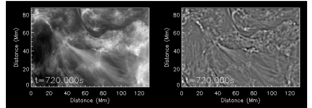
Fig. A.5. Still from Movie 4. The movie is of the same coronal structure as in Movie 3 but observed with AIA 193 Å. The field of view covers a slightly large region than that of Movie 3. The time period corresponding to the Hi-C data is from 660 s to 870 s.
