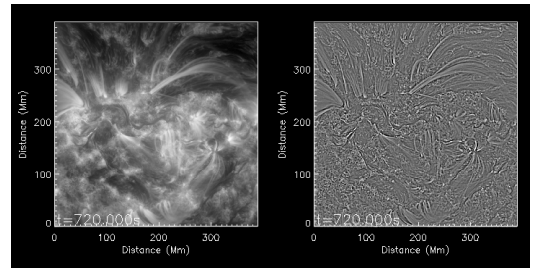
Fig. A.6. Still from Movie 5, showing the region observed by AIA 171 Å that is displayed in Fig. 1 in the main text. The coronal structures labelled A, B, 1, 2 and 3 are all visible in the movie. Note the visible motion in feature 3, in which the analysis finds relatively large velocity amplitude ( >5 km s ^{-1} ) transverse displacements. This is compared with the other structures, where our analysis revealed only small velocity amplitudes.
