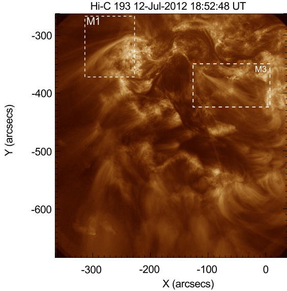
Fig. A.1. Active region as observed with Hi-C 193 Å. Movie 1 (M1) focuses on the coronal structure labelled A in the main text and parts Movie 3 (M3) focuses on the coronal structure labelled B in the manuscript. The boxes show the sub-regions of the Hi-C field of view in each movie.
