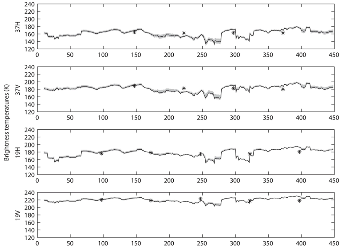
Figure 7 – HUT brightness temperature simulations, after application of grain scaling factors, using all extinction coefficients models (mean - black line; range - shaded grey area) and measured brightness temperatures (asterisks).
