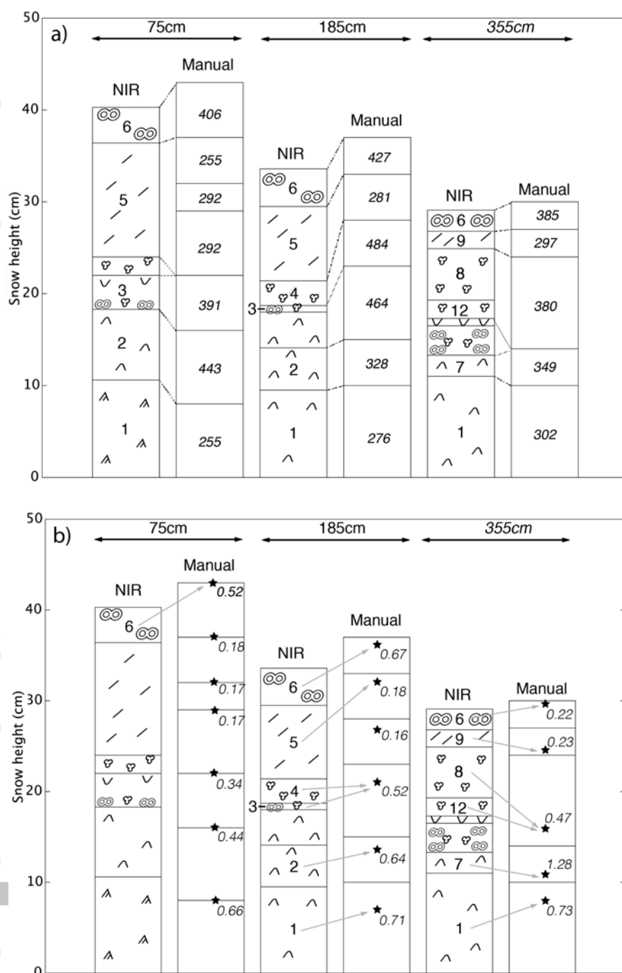
Figure 3 – a) Translating densities (in \text{kg m}^{-3} ) from manual vertical profiles to NIR layers, b) Translating effective grain diameters (in mm) from manual vertical profiles to NIR layers, stars represent the location of measurements within the profiles. Symbols describe snow type following the classification of Fierz et al. (2009).
